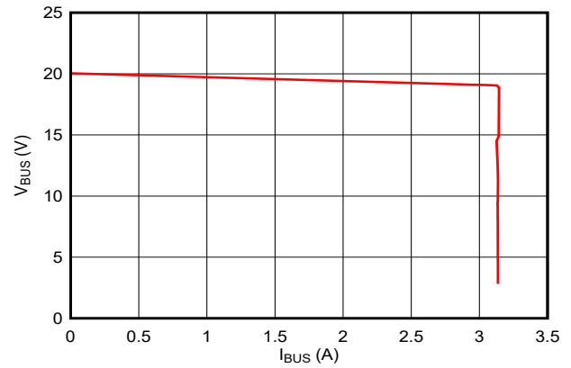
Figure 7-32. Constant Voltage to Constant Current Transition V_{IN} = 13.5\text{ V} V_{BUS} = 20\text{ V (CV)} I_{LIMIT} = 3.15\text{ A (CC)}
