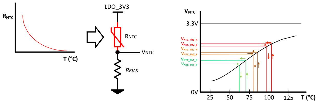
Figure 9-42. NTC Response Curve
