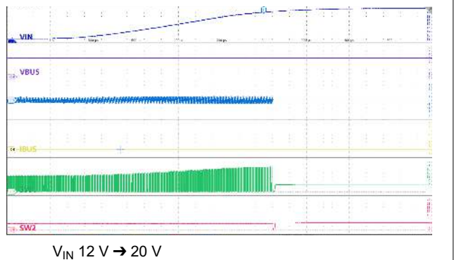
Figure 10-27. V_{IN(OVP)} Entry
