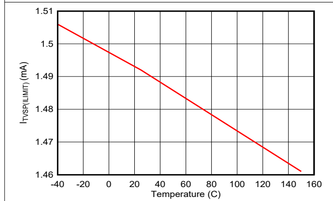
Figure 7-15. I_{TVSP(ILIMIT)} vs Temperature
