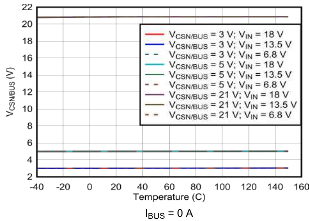
Figure 7-33. Buck-boost Output Voltage Regulation vs Temperature I_{BUS} = 0\text{ A}
