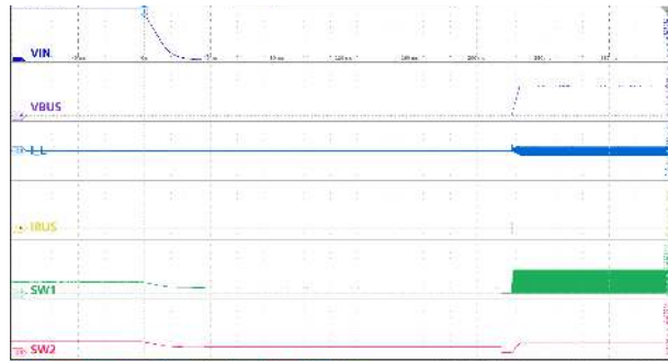
Figure 10-28. V_{IN(OVP)} Recovery
