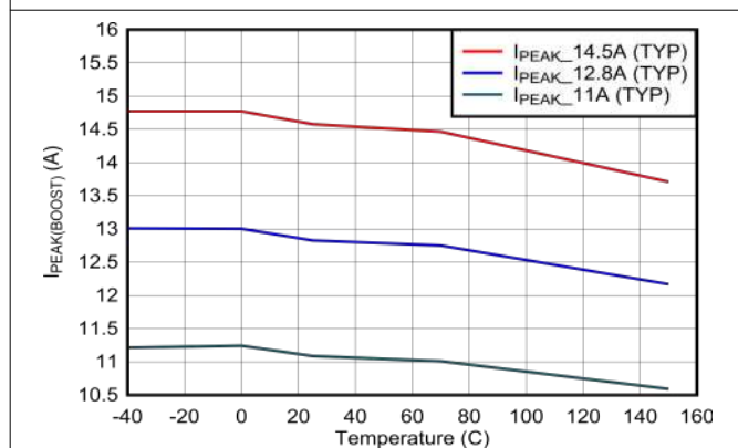
Figure 7-17. Boost Peak Current Limit vs Temperature (upper settings)
