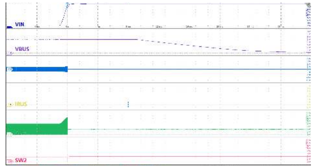
Figure 10-29. V_{IN(OVP)} Showing V_{BUS} Discharge
