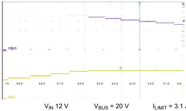
V_{IN} = 12\text{ V} V_{BUS} = 20\text{ V} I_{LIMIT} = 3.1\text{ A} Figure 10-34. Current Limit: Stepped Resistive Load
