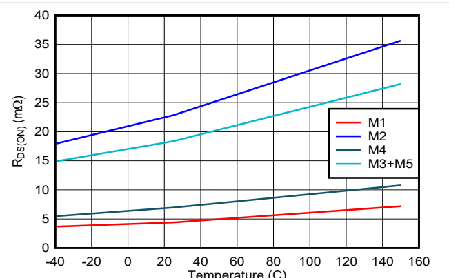
Figure 7-16. Buck-Boost Power FET R_{DS(ON)} vs Temperature
