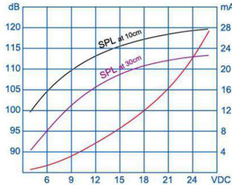
SPL & Current Consumption vs. Input Voltage
