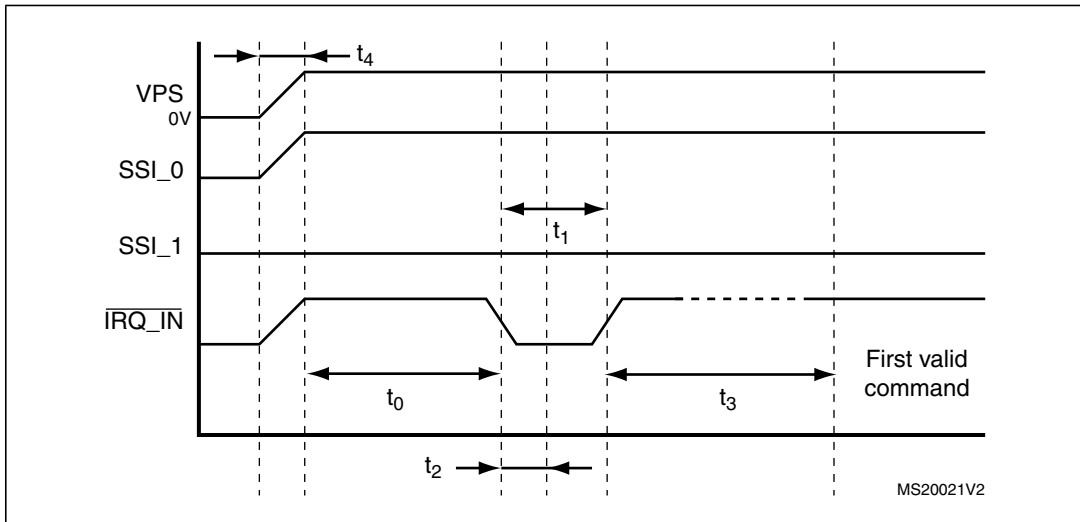
Figure 5. Power-up sequence
