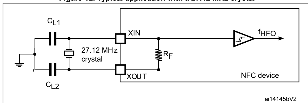
Figure 12. Typical application with a 27.12 MHz crystal
