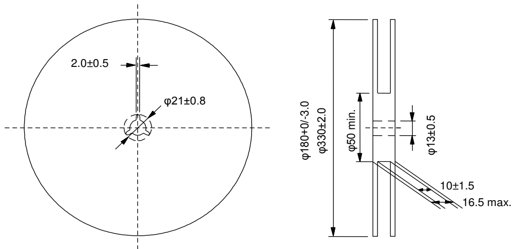
Fig.3 Taping Diagram
