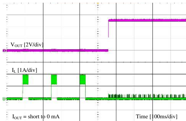
Figure 9-9. Short Recovery
