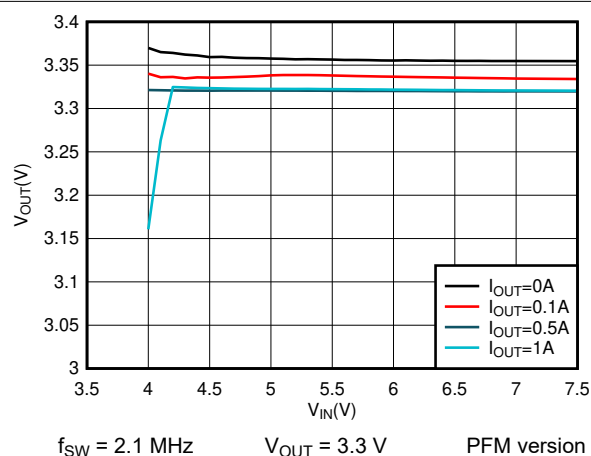
Figure 7-6. 3.3-V Dropout
