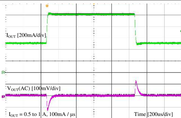
Figure 9-7. Load Transient
