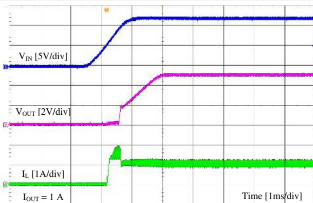
Figure 9-5. Start Up by V_{IN}
