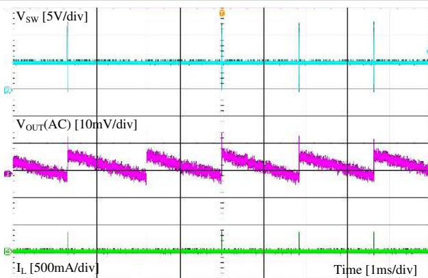
Figure 9-3. Ripple at No Load
