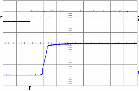
Fig. 1.5V.7: Turn-on transient at full rated load current (resistive) with no output capacitor at V_{in} = 48\text{ V} , triggered via ON/OFF pin. Top trace: ON/OFF signal (5 V/div.). Bottom trace: output voltage (0.5 V/div.) Time scale: 2 ms/div.
