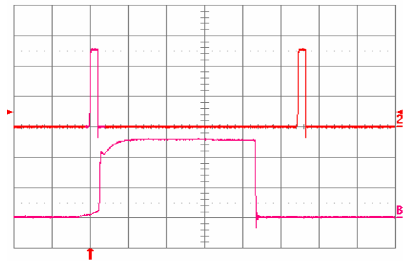
Fig. 1.5V.15: Load current (top trace, 20 A/div, 20 ms/div) into a 10 m\Omega short circuit during restart, at V_{in} = 48 V. Bottom trace (20 A/div, 1 ms/div) is an expansion of the on-time portion of the top trace.
