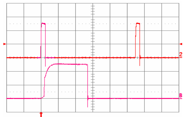
Fig. 1.8V.15: Load current (top trace, 20 A/div, 20 ms/div) into a 10 m\Omega short circuit during restart, at V_{in} = 48 V. Bottom trace (20 A/div, 2 ms/div) is an expansion of the on-time portion of the top trace.
