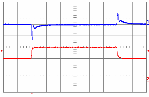
Fig. 1.2V.9: Output voltage response to load current step-change (20 A – 30 A – 20 A) at V_{in} = 48\text{ V} . Top trace: output voltage (100 mV/div.). Bottom trace: load current (10 A/div). Current slew rate: 1 A/ \mu\text{s} . C_o = 470\text{ }\mu\text{F} tantalum + 1 \mu\text{F} ceramic. Time scale: 0.2 ms/div.
