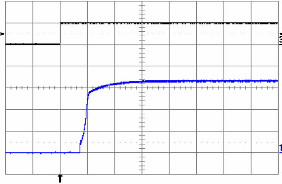
Fig. 1.8V.7: Turn-on transient at full rated load current (resistive) with no output capacitor at V_{in} = 48 V, triggered via ON/OFF pin. Top trace: ON/OFF signal (5 V/div.). Bottom trace: output voltage (1 V/div.) Time scale: 2 ms/div.
