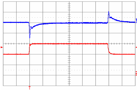
Fig. 1.5V.9: Output voltage response to load current step-change (20 A – 30 A – 20 A) at V_{in} = 48\text{ V} . Top trace: output voltage (100 mV/div.). Bottom trace: load current (10 A/div). Current slew rate: 1 A/ \mu\text{s} . C_o = 470\text{ }\mu\text{F} tantalum + 1 \mu\text{F} ceramic. Time scale: 0.2 ms/div.
