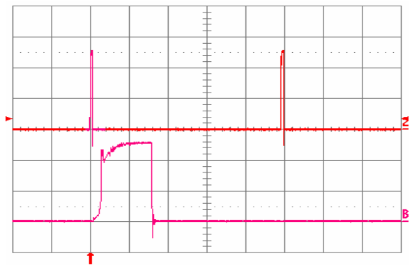
Fig. 3.3V.15: Load current (top trace, 20 A/div, 20 ms/div) into a 10 m\Omega short circuit during restart, at V_{in} = 48 V. Bottom trace (20 A/div, 1 ms/div) is an expansion of the on-time portion of the top trace.
