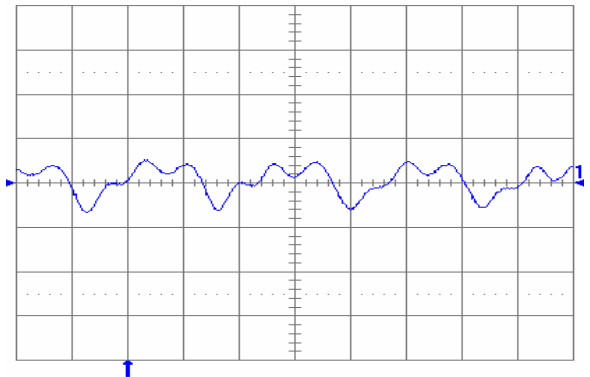
Fig. 2.0V.10: Output voltage ripple (20 mV/div.) at full rated load current into a resistive load with C_o = 10\ \mu\text{F} tantalum + 1 \mu\text{F} ceramic and V_{in} = 48\text{ V} . Time scale: 1 \mu\text{s} /div.
