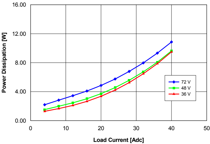
Fig. 1.2V.5: Power dissipation vs. load current and input voltage for converter mounted vertically with air flowing from pin 3 to pin 1 at a rate of 300 LFM (1.5 m/s) and T_a = 25\text{ }^\circ\text{C} .
