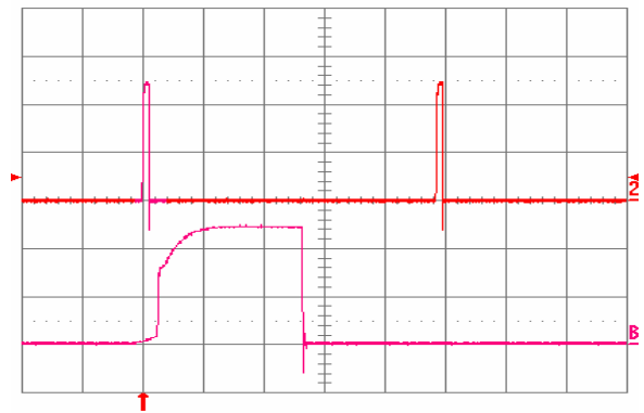
Fig. 2.0V.15: Load current (top trace, 20 A/div, 20 ms/div) into a 10 m\Omega short circuit during restart, at V_{in} = 48 V. Bottom trace (20 A/div, 1 ms/div) is an expansion of the on-time portion of the top trace.
