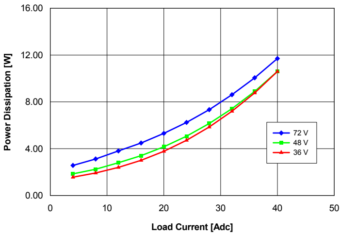
Fig. 1.8V.5: Power dissipation vs. load current and input voltage for converter mounted vertically with air flowing from pin 3 to pin 1 at a rate of 300 LFM (1.5 m/s) and T_a = 25\text{ }^\circ\text{C} .
