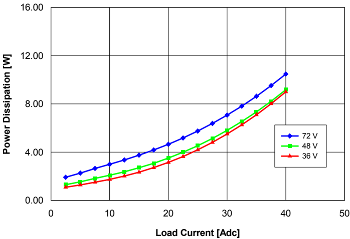
Fig. 1.0V.5: Power dissipation vs. load current and input voltage for converter mounted vertically with air flowing from pin 3 to pin 1 at a rate of 300 LFM (1.5 m/s) and T_a = 25\text{ }^\circ\text{C} .
