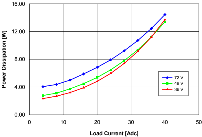
Fig. 3.3V.5: Power dissipation vs. load current and input voltage for converter mounted vertically with air flowing from pin 3 to pin 1 at a rate of 300 LFM (1.5 m/s) and T_a = 25\text{ }^\circ\text{C} .
