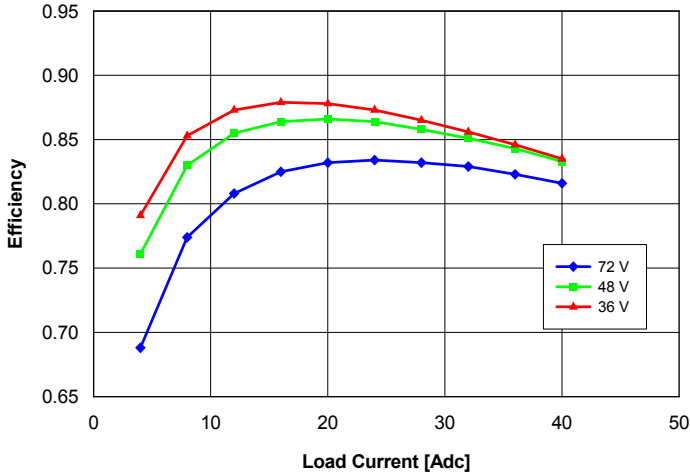
Fig. 1.2V.3: Efficiency vs. load current and input voltage for converter mounted vertically with air flowing from pin 3 to pin 1 at a rate of 300 LFM (1.5 m/s) and T_a = 25\text{ }^\circ\text{C} .
