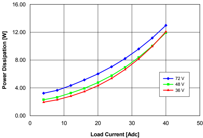
Fig. 2.5V.5: Power dissipation vs. load current and input voltage for converter mounted vertically with air flowing from pin 3 to pin 1 at a rate of 300 LFM (1.5 m/s) and T_a = 25\text{ }^\circ\text{C} .
