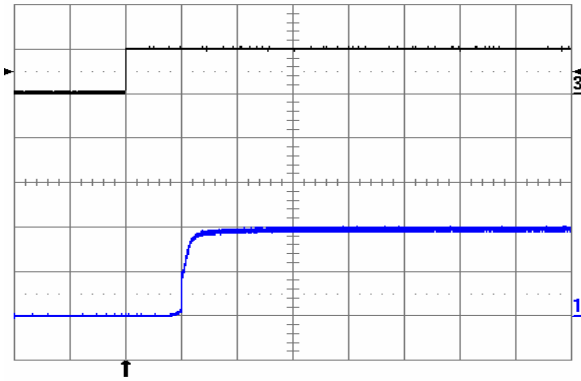
Fig. 1.0V.7: Turn-on transient at full rated load current (resistive) with no output capacitor at V_{in} = 48\text{ V} , triggered via ON/OFF pin. Top trace: ON/OFF signal (5 V/div.). Bottom trace: output voltage (0.5 V/div.) Time scale: 2 ms/div.
