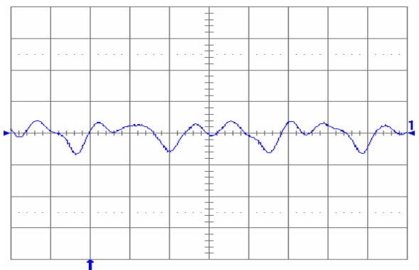
Fig. 1.2V.10: Output voltage ripple (20 mV/div.) at full rated load current into a resistive load with C_o = 10\text{ }\mu\text{F} tantalum + 1 \mu\text{F} ceramic and V_{in} = 48\text{ V} . Time scale: 1 \mu\text{s} /div.
