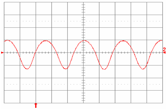
Fig. 1.5V.13: Input reflected ripple current, i_c (100 mA/div), measured at input terminals at full rated load current and V_{in} = 48 V. Refer to Fig. 1.5V.11 for test setup. Time scale: 1 \mu s/div.
