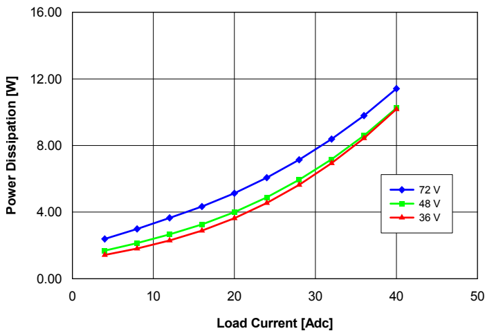
Fig. 1.5V.5: Power dissipation vs. load current and input voltage for converter mounted vertically with air flowing from pin 3 to pin 1 at a rate of 300 LFM (1.5 m/s) and T_a = 25\text{ }^\circ\text{C} .
