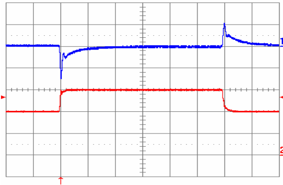
Fig. 1.8V.9: Output voltage response to load current step-change (20 A – 30 A – 20 A) at V_{in} = 48 V. Top trace: output voltage (100 mV/div.). Bottom trace: load current (10 A/div). Current slew rate: 1 A/ \mu s. C_o = 470 \mu F tantalum + 1 \mu F ceramic. Time scale: 0.2 ms/div.
