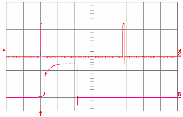
Fig. 2.5V.15: Load current (top trace, 20 A/div, 20 ms/div) into a 10 m\Omega short circuit during restart, at V_{in} = 48 V. Bottom trace (20 A/div, 1 ms/div) is an expansion of the on-time portion of the top trace.
