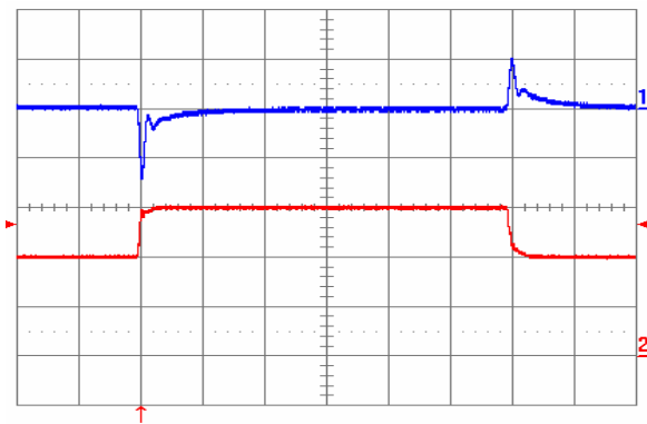
Fig. 1.0V.9: Output voltage response to load current step-change (20 A – 30 A – 20 A) at V_{in} = 48\text{ V} . Top trace: output voltage (100 mV/div.). Bottom trace: load current (10 A/div). Current slew rate: 1 A/ \mu\text{s} . C_o = 470\text{ }\mu\text{F} tantalum + 1 \mu\text{F} ceramic. Time scale: 0.2 ms/div.
