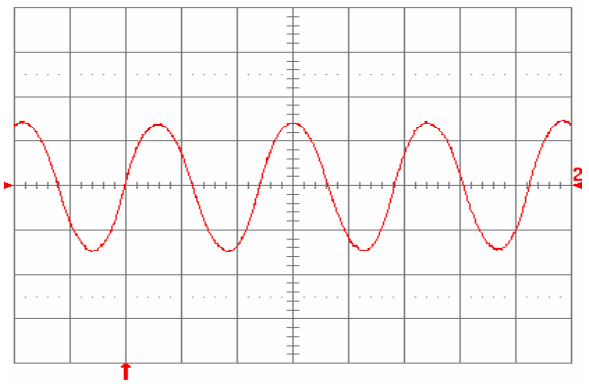
Fig. 2.5V.13: Input reflected ripple current, i_c (100 mA/div), measured at input terminals at full rated load current and V_{in} = 48 V. Refer to Fig. 2.5V.11 for test setup. Time scale: 1 \mu s/div.
