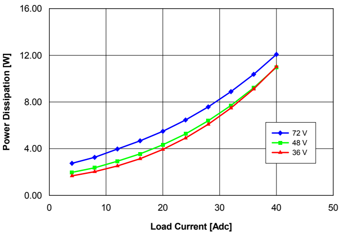
Fig. 2.0V.5: Power dissipation vs. load current and input voltage for converter mounted vertically with air flowing from pin 3 to pin 1 at a rate of 300 LFM (1.5 m/s) and T_a = 25\text{ }^\circ\text{C} .
