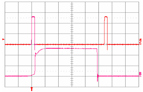
Fig. 1.2V.15: Load current (top trace, 20 A/div, 20 ms/div) into a 10 m\Omega short circuit during restart, at V_{in} = 48 V. Bottom trace (20 A/div, 1 ms/div) is an expansion of the on-time portion of the top trace.
