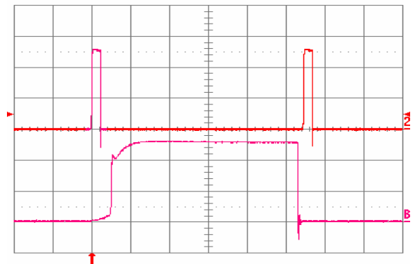
Fig. 1.0V.15: Load current (top trace, 20 A/div, 20 ms/div) into a 10 m\Omega short circuit during restart, at V_{in} = 48 V. Bottom trace (20 A/div, 1 ms/div) is an expansion of the on-time portion of the top trace.
