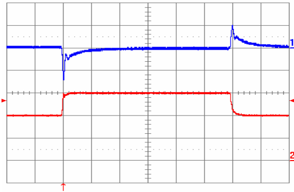
Fig. 2.5V.9: Output voltage response to load current step-change (20 A – 30 A – 20 A) at V_{in} = 48\text{ V} . Top trace: output voltage (100 mV/div.). Bottom trace: load current (10 A/div). Current slew rate: 1 A/ \mu\text{s} . C_o = 470\text{ }\mu\text{F} tantalum + 1 \mu\text{F} ceramic. Time scale: 0.2 ms/div.
