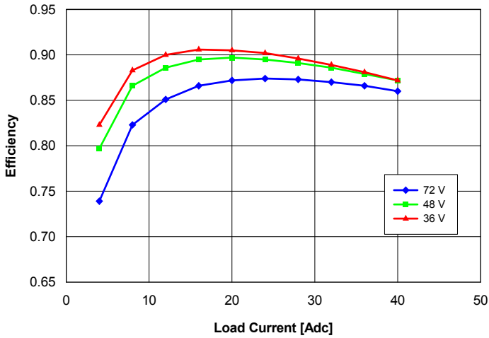
Fig. 1.8V.3: Efficiency vs. load current and input voltage for converter mounted vertically with air flowing from pin 3 to pin 1 at a rate of 300 LFM (1.5 m/s) and T_a = 25\text{ }^\circ\text{C} .
