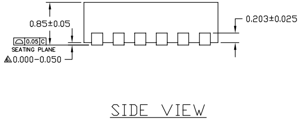
17-Pin 2.5mm x 2.8mm MLF® (ML)
