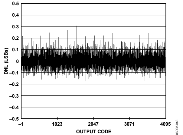
Figure 43. AD9230-250 DNL; 250 MSPS
