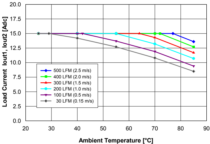
Fig. 10: Available balanced load current ( I_{out1} = I_{out2} ) vs. ambient air temperature and airflow rates for converter with D height pins mounted vertically with V_{in} = 48\text{ V} , air flowing from pin 3 to pin 1 and maximum FET temperature \leq 120^\circ\text{C} .
