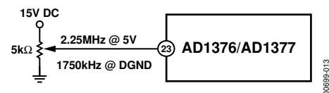
Figure 13. Clock Rate Control Circuit
