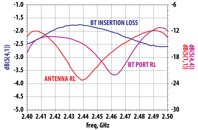
Figure 8. BT Path 2.4 – 2.5 GHz Insertion Loss and Return Loss
