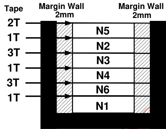
Bobbin
