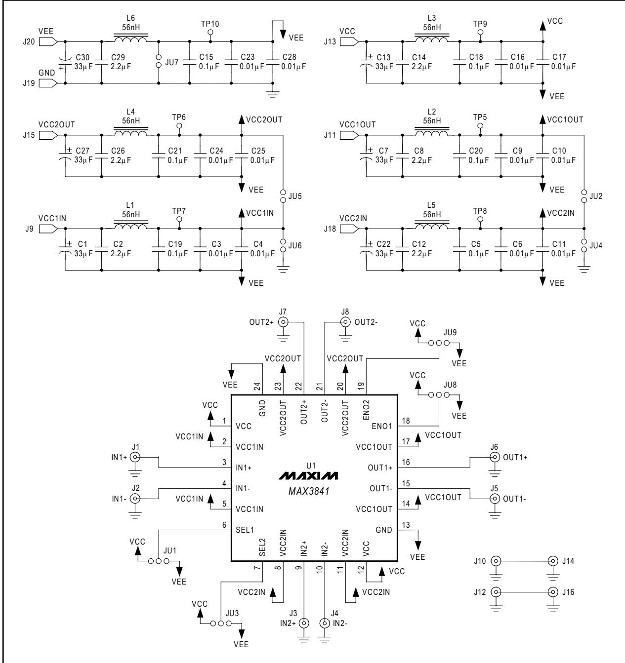
Figure 1. MAX3841 EV Kit Schematic Diagram
