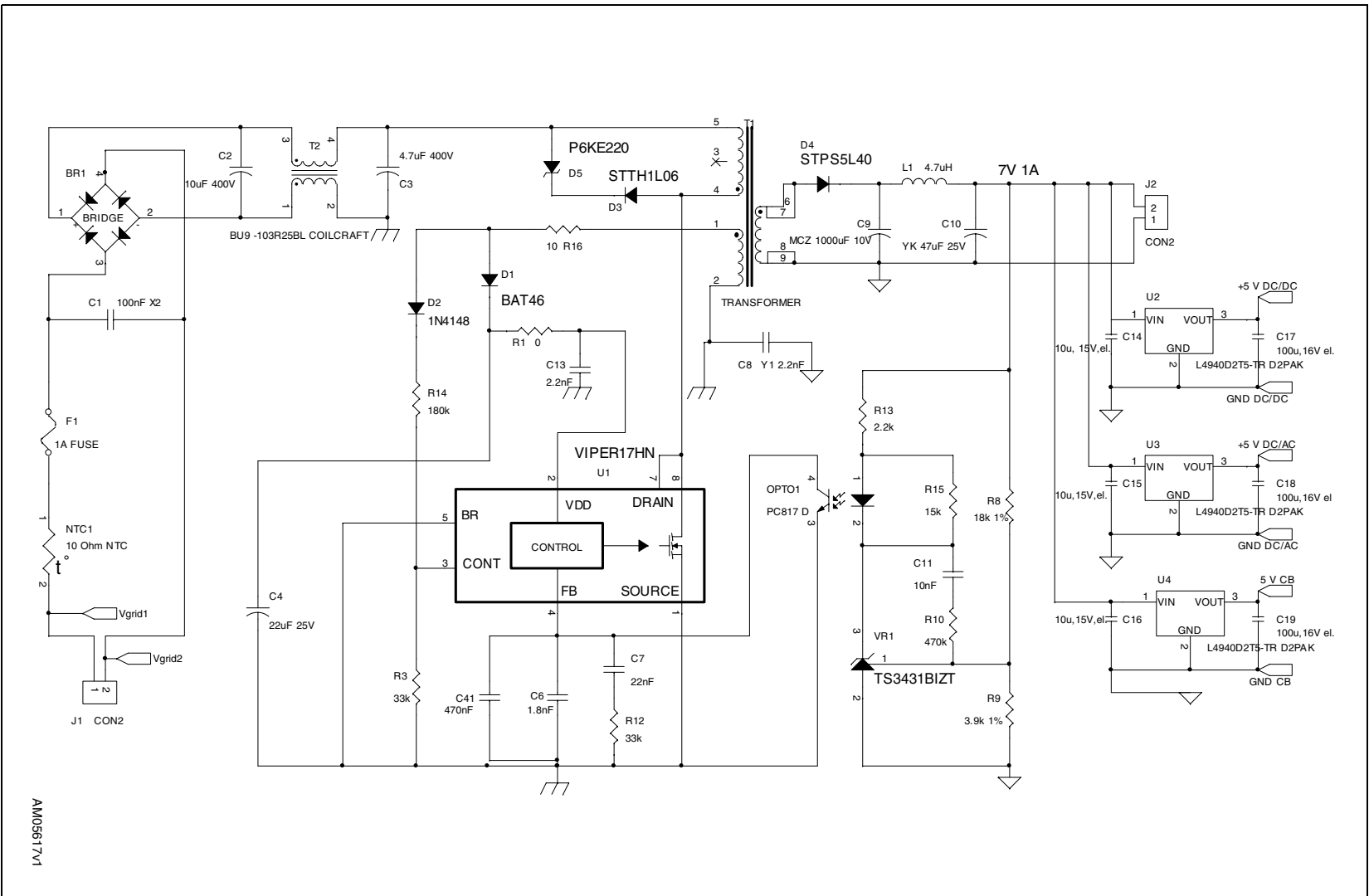
Figure 9. Multi-output flyback converter with VIPER27HN schematic
