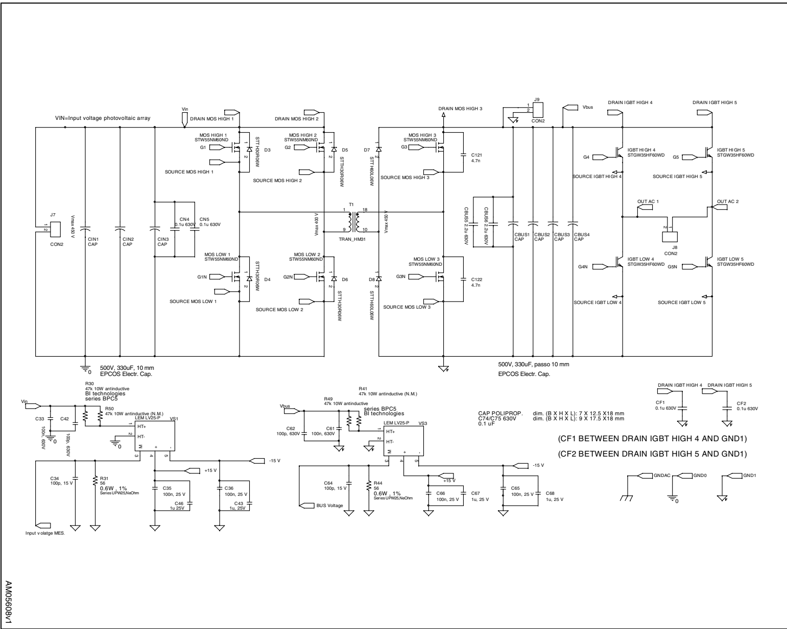
Figure 1. STEVAL-ISV002V1 power stage circuit schematic
