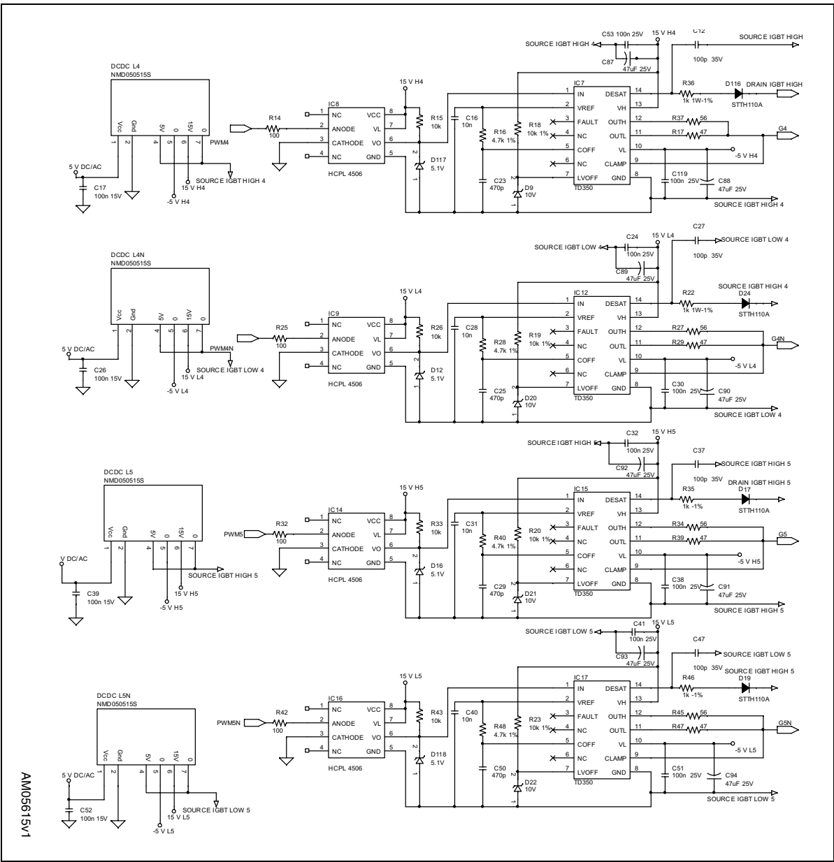
Figure 7. DC-AC converter driver circuit schematic
