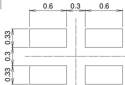
PCB Pattern
