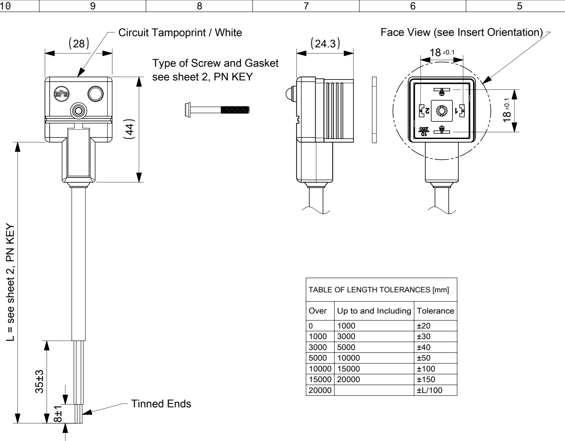
Type of Screws and Gaskets
