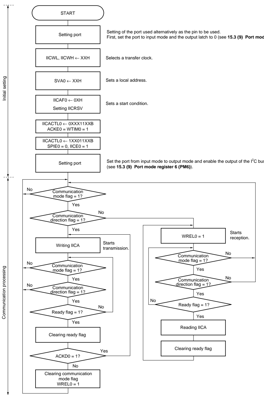
Figure 15-31. Slave Operation Flowchart (1)
