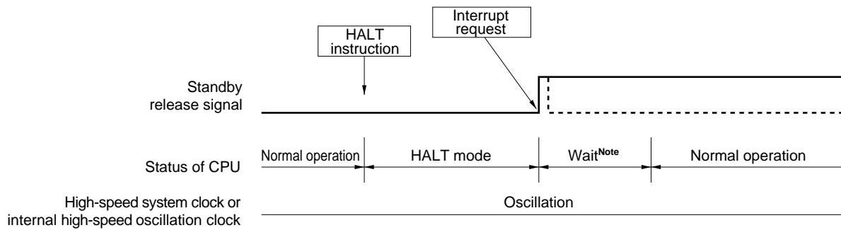
Figure 19-3. HALT Mode Release by Interrupt Request Generation
