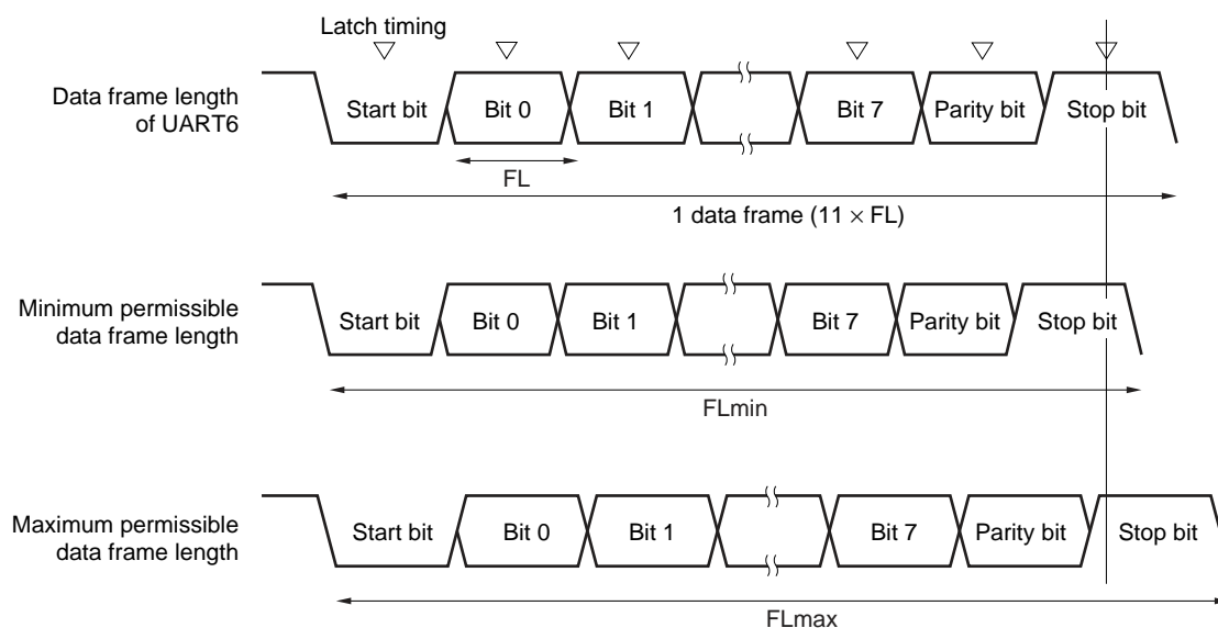
Figure 14-35. Permissible Baud Rate Range During Reception
