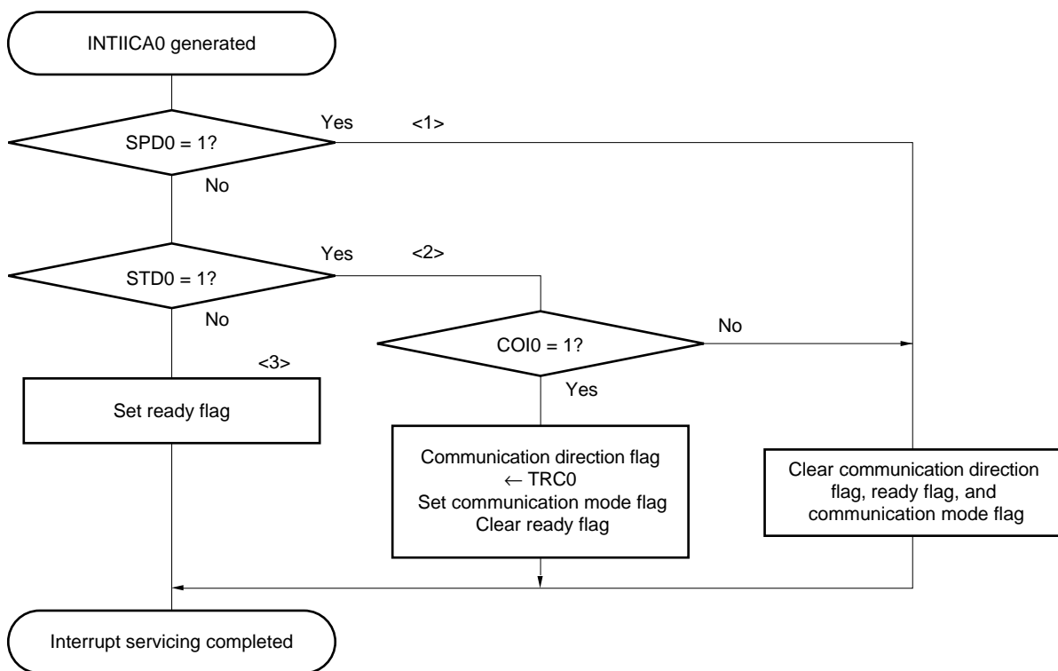
Figure 15-32. Slave Operation Flowchart (2)
