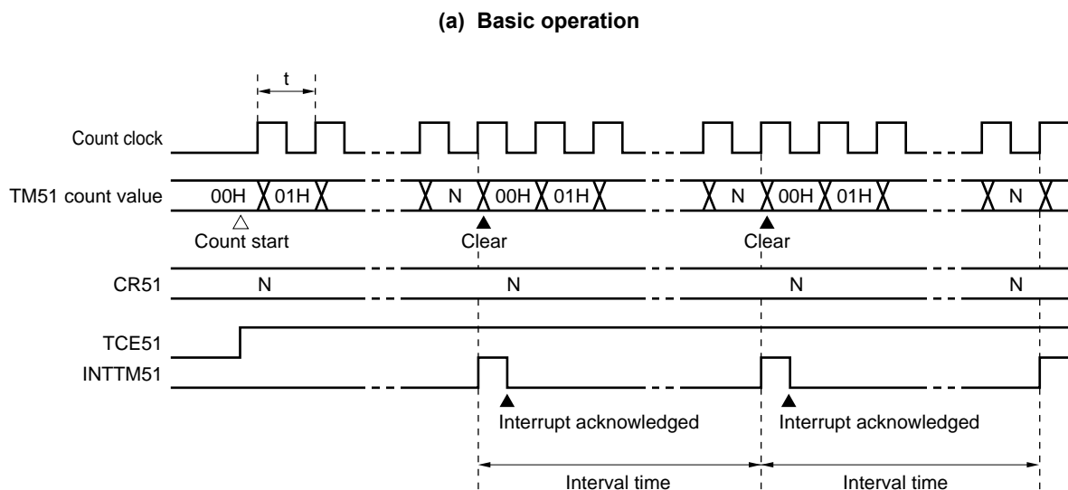
Figure 8-9. Interval Timer Operation Timing (1/2)
