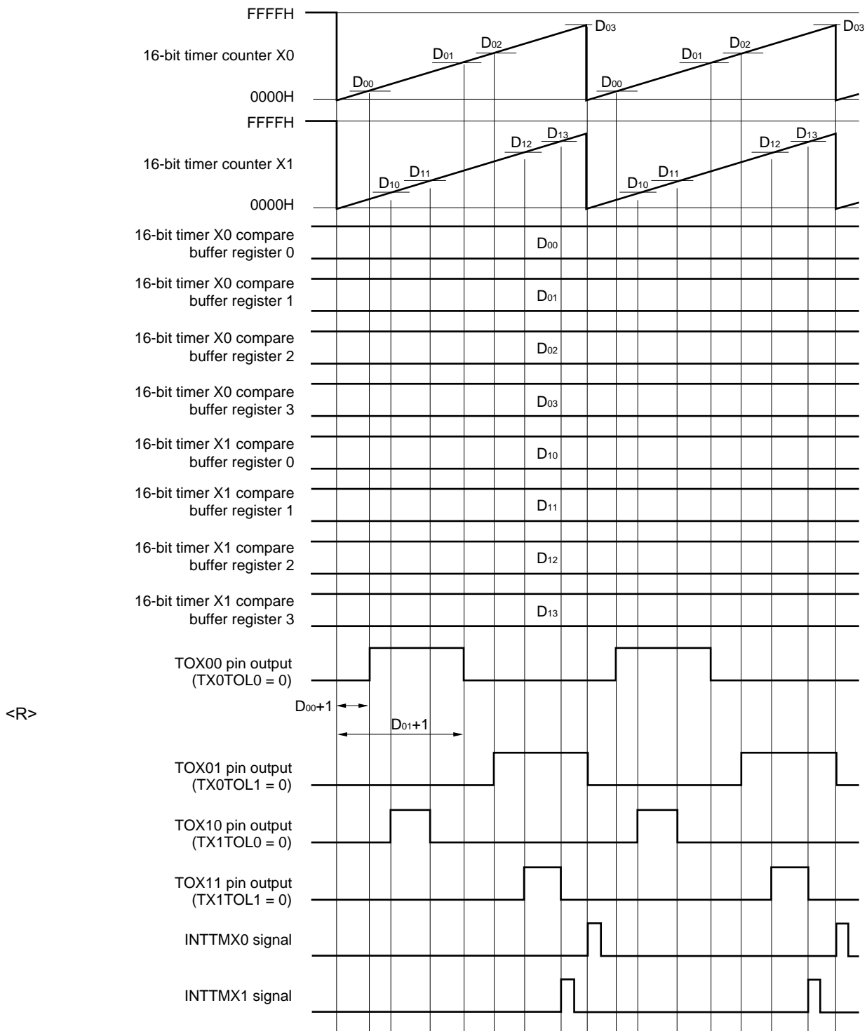
Figure 6-34. PWM Output Timing (Synchronous start/clear mode, TMX0 dual output, TMX1 dual output)
