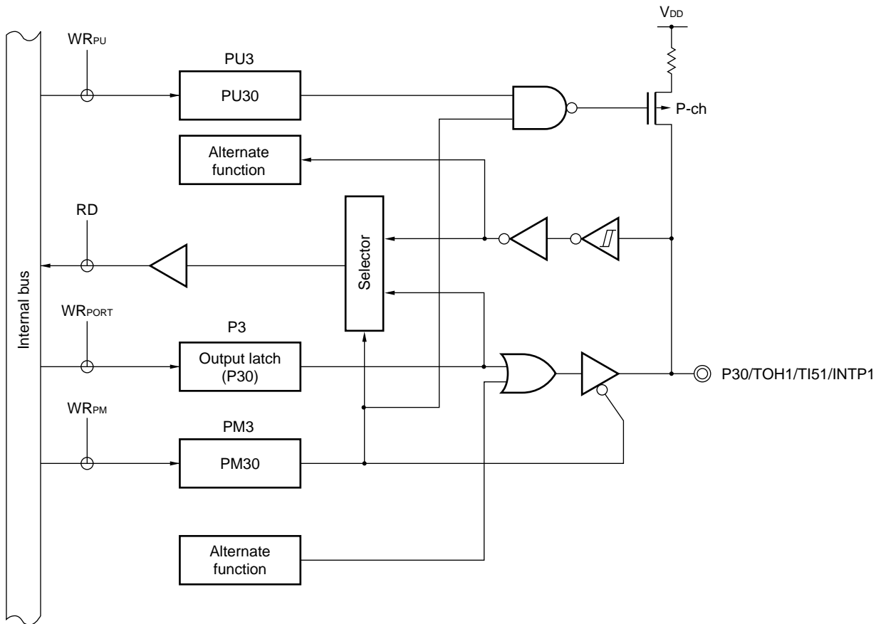
Figure 4-12. Block Diagram of P30
