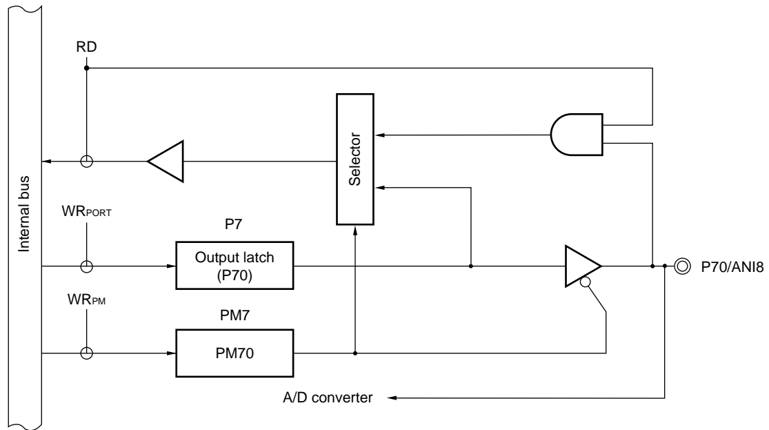
Figure 4-22. Block Diagram of P70
