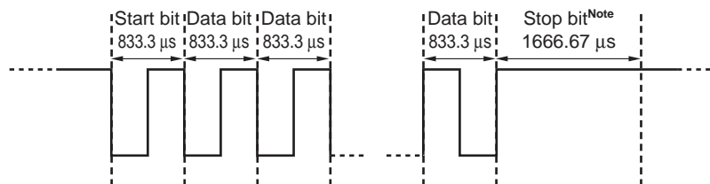
Figure 14-29. Timing in the Frame
