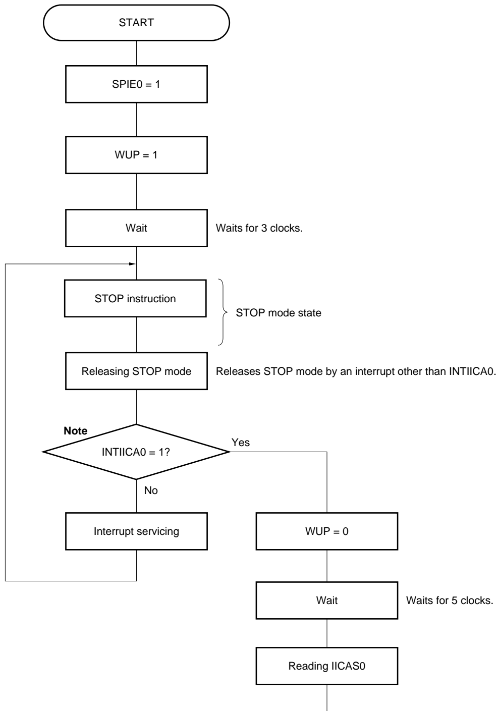
Figure 15-25. When Releasing STOP Mode other than by INTIICA0
