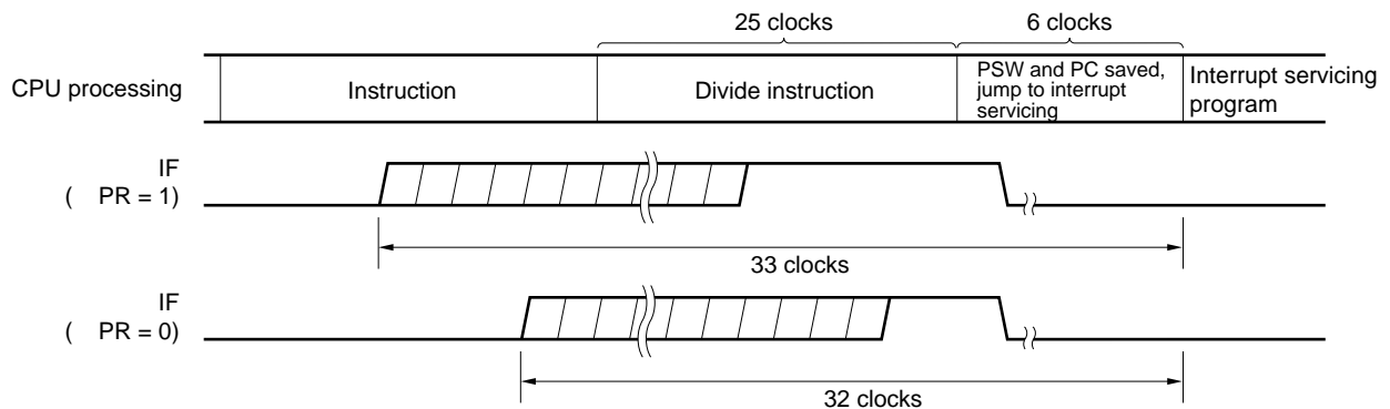
Figure 18-16. Interrupt Request Acknowledgment Timing (Maximum Time)
