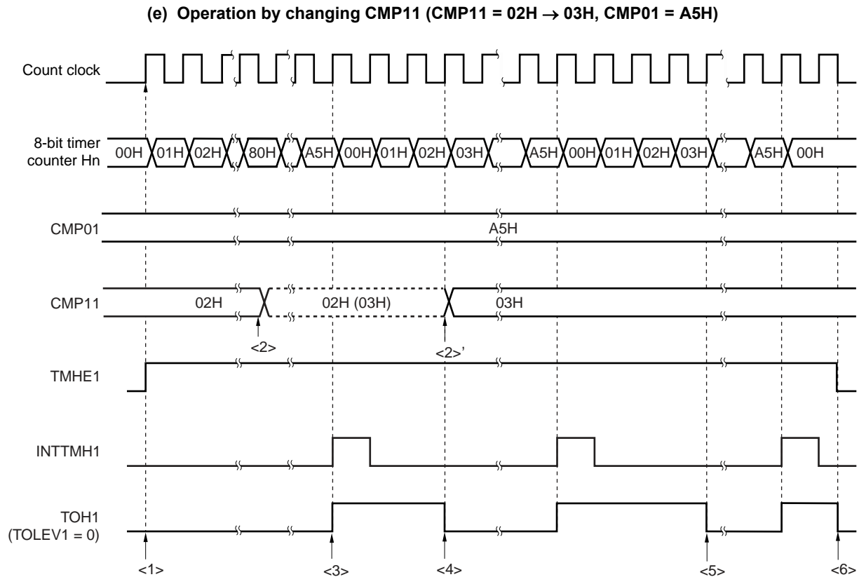
Figure 9-12. Operation Timing in PWM Output Mode (4/4)
