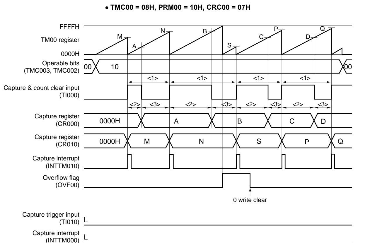
Figure 7-51. Timing Example of Pulse Width Measurement (3)
