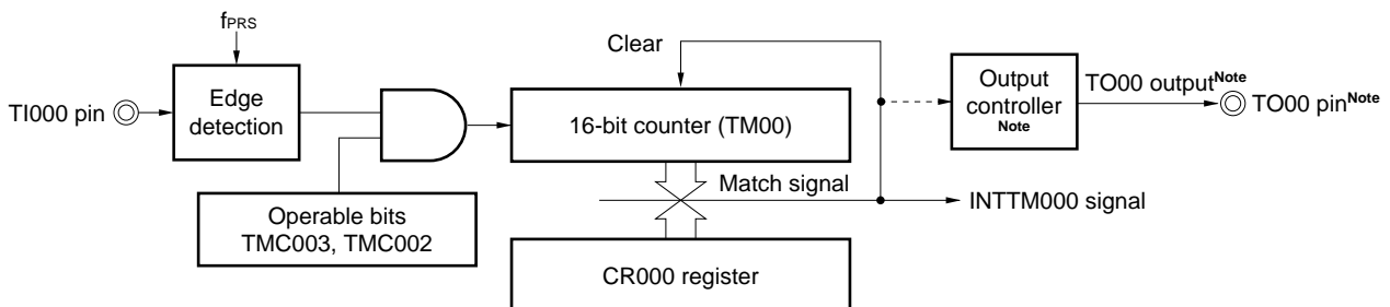
Figure 7-20. Block Diagram of External Event Counter Operation
