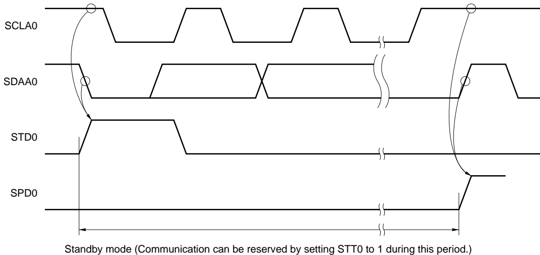
Figure 15-27. Timing for Accepting Communication Reservations
