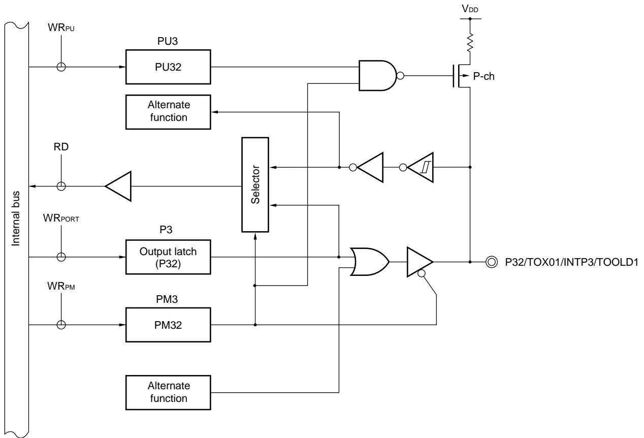
Figure 4-14. Block Diagram of P32
