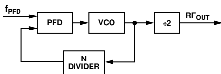
Figure 32. Loop Closed Before Output Divider
