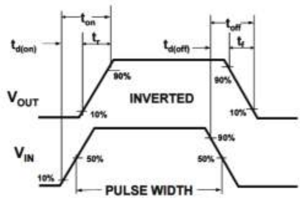
Figure8. Switching wave
