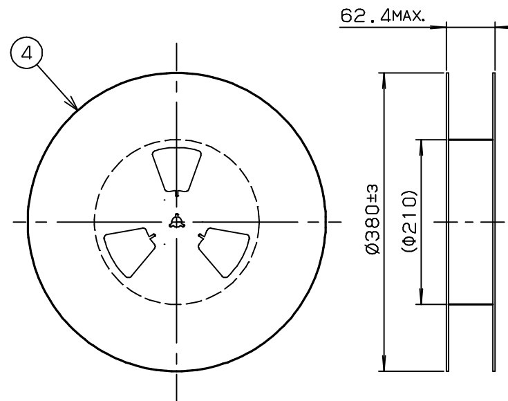
REEL DIMENSION
