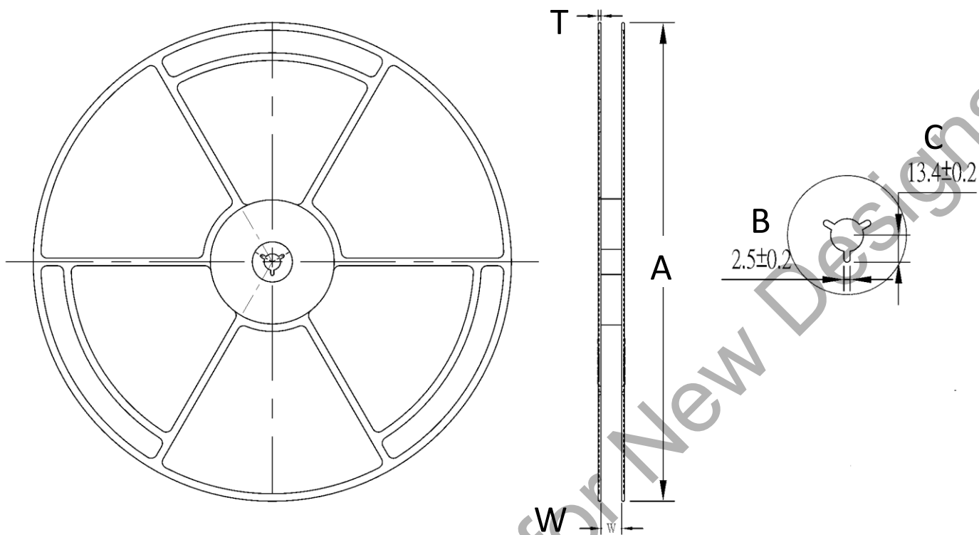
Figure 8 - Reel Specifications
