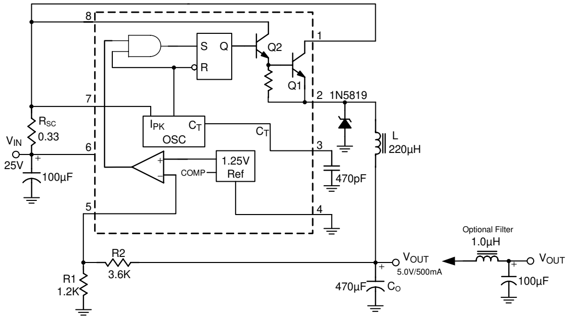
Figure 3. Step-down Converter
