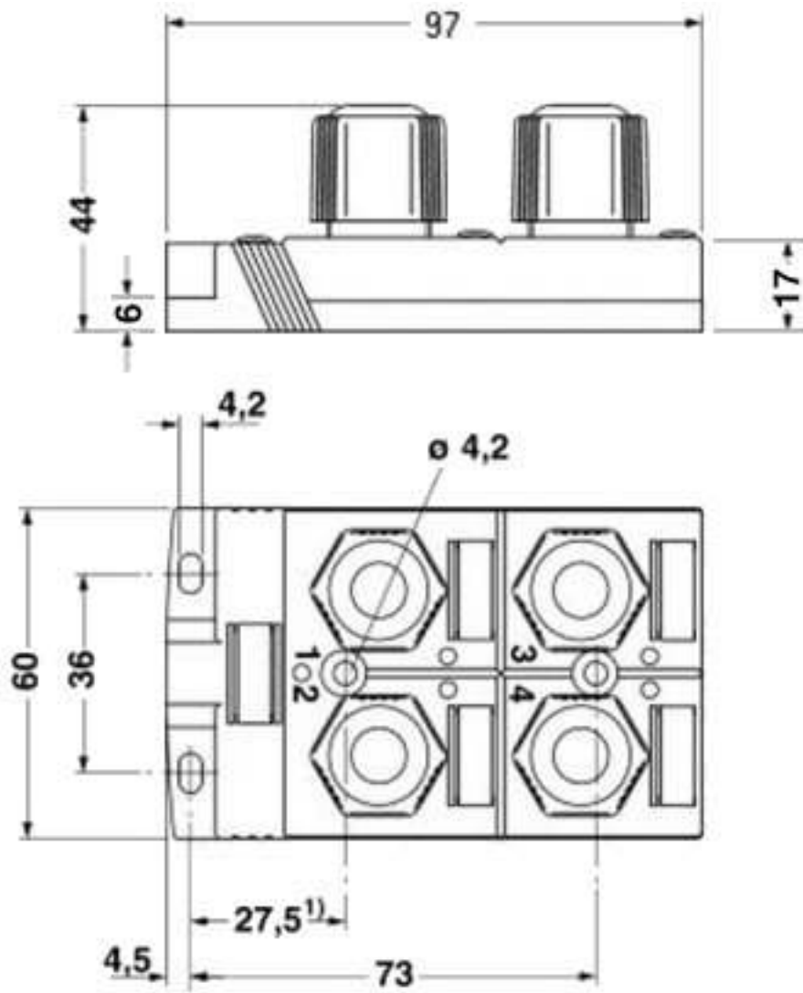
Dimensioned drawing
