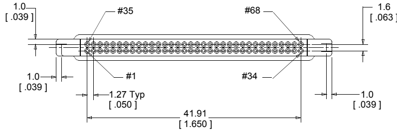
PC Card Socket Interface View 2:1
