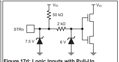
Figure 17d: Logic Inputs with Pull-Up
