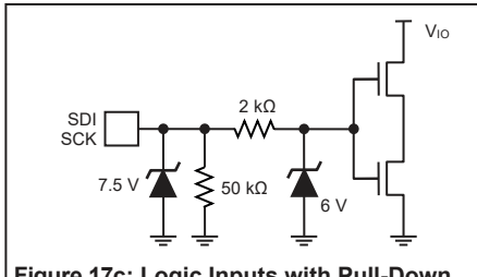
Figure 17c: Logic Inputs with Pull-Down
