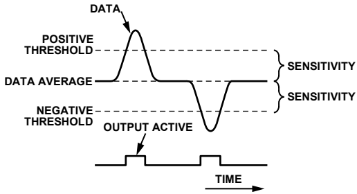
Figure 29. Threshold Sensitivity
