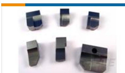
TE Part #1803426-2 ANVIL, COMBINATION, NO JOG, END FEED
