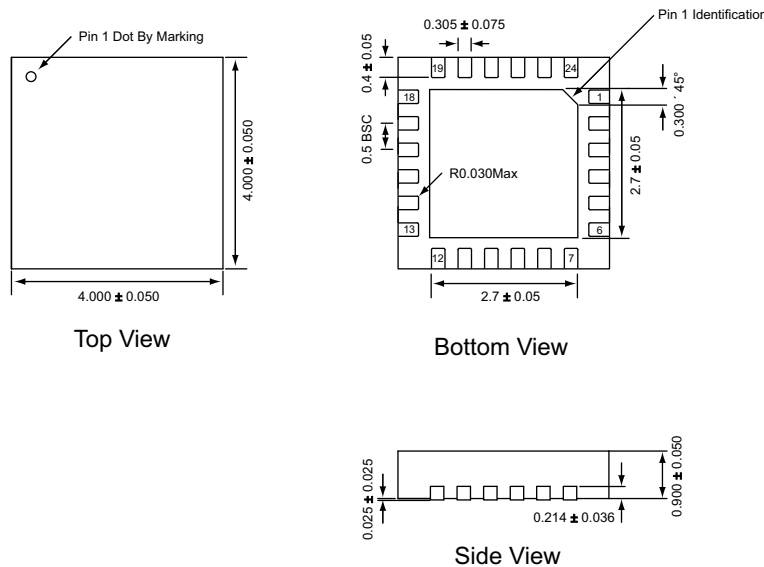
QFN44-24
