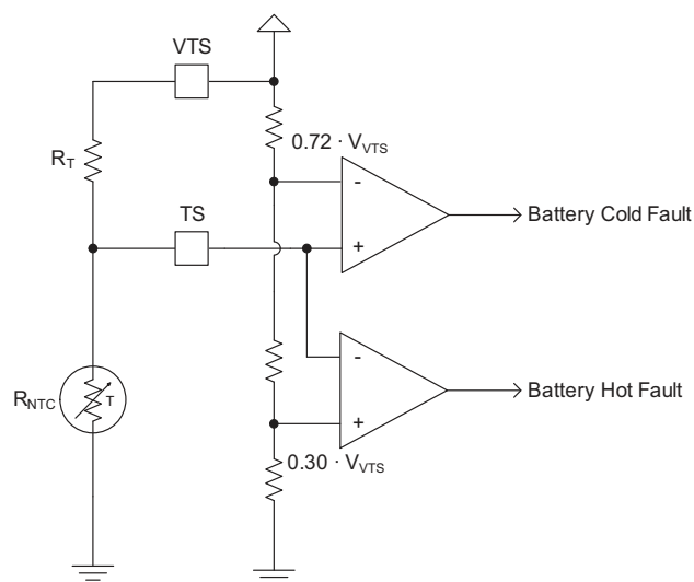
Figure 6: Battery Temperature Sense Circuit.
