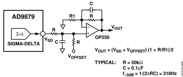
Figure 9. Σ-Δ Active Filter with Gain and Offset
