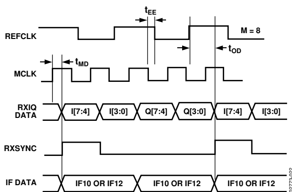
Figure 22. Rx Port Timing (Nonmultiplexed Data)
