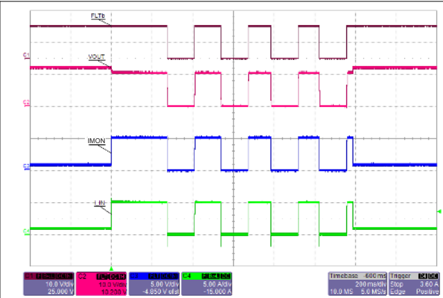
Figure 10-12. Overload Condition: Auto Retry and Recovery - TPS25940-Q1
