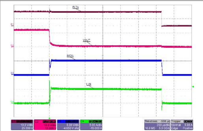
Figure 10-18. Hot Short: Latched - TPS25940L-Q1
