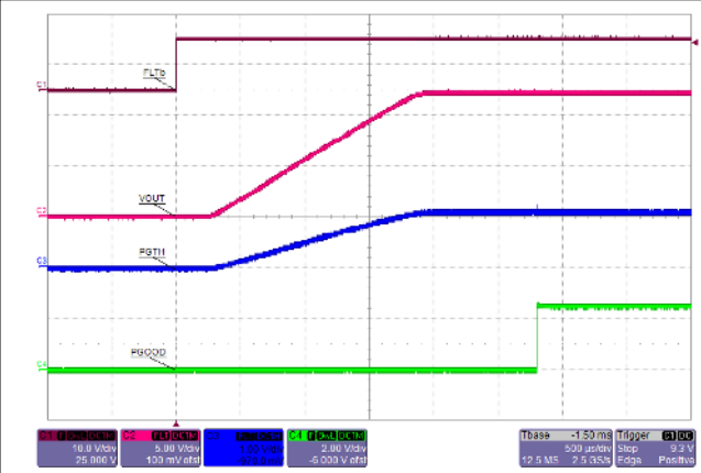
Figure 10-16. Power Good Response During Turn-ON
