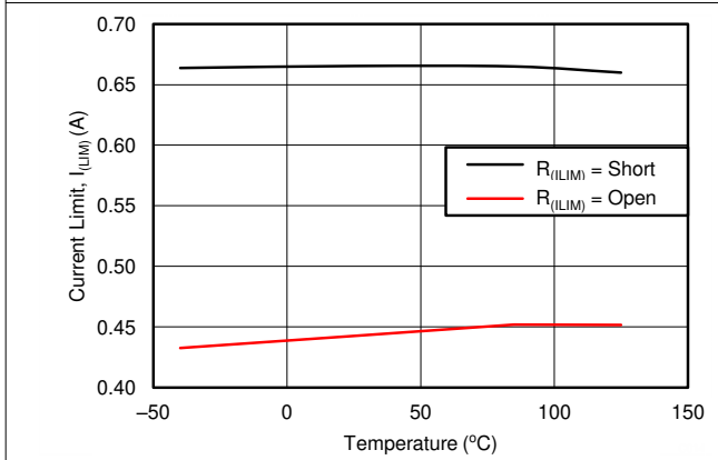
Figure 7-21. Current Limit for R_{(LIM)} = \text{Open} and Short vs Temperature
