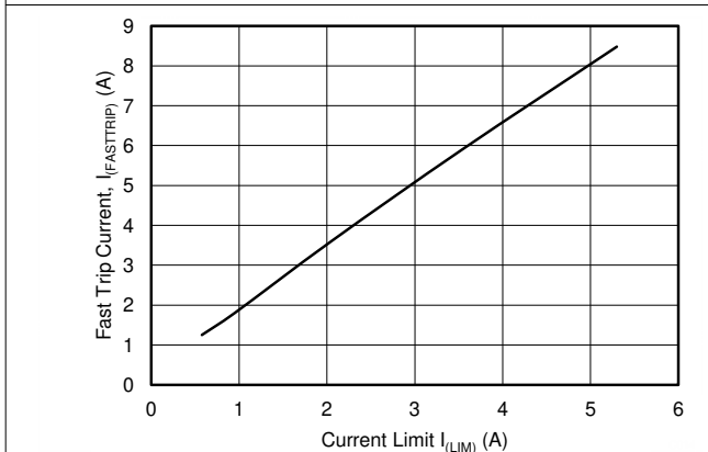
Figure 7-23. Fast Trip Threshold vs Current Limit
