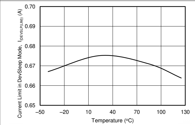
Figure 7-22. Current Limit in DevSleep Mode vs Temperature
