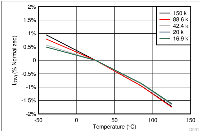
Figure 7-19. Current Limit (% Normalized) vs R_{(LIMIT)} Resistor
