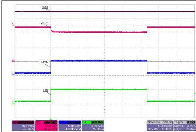
Figure 10-11. Over Load: Step Change in Load from 12 \Omega to 2 \Omega and Back
