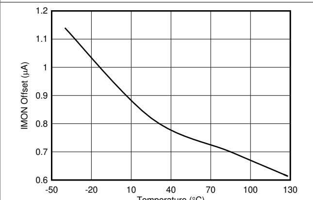
Figure 7-24. IMON Offset vs Temperature
