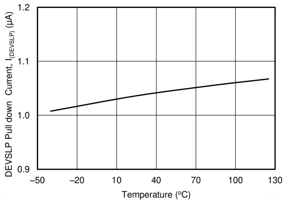
Figure 7-13. DEVSLEP Pull Down Current vs Temperature
