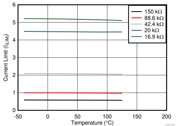
Figure 7-18. Current Limit vs Temperature Across R (ILIM)
