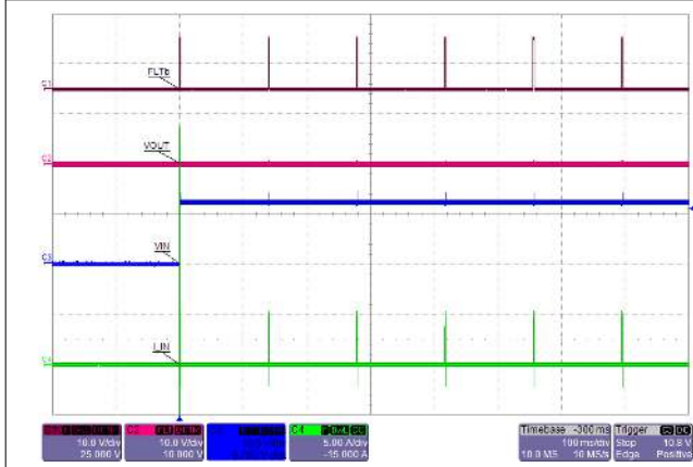
Figure 10-15. Hot Plug-In with Short on Output: Auto-Retry - TPS25940-Q1
