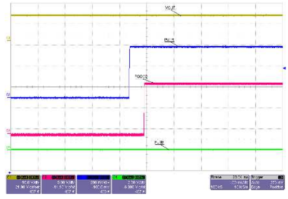
V_{(IN)} = 12\text{ V} R_L = 12\text{ }\Omega R_{(FLT)} = 100\text{ k}\Omega Figure 7-38. Power Good Delay (Rising)
