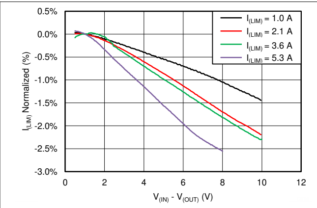
Figure 7-20. Current Limit Normalized (%) vs V_{(IN)} - V_{(OUT)}
