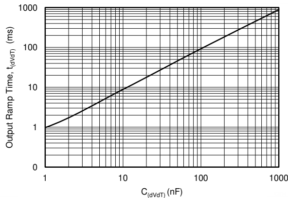
Figure 7-15. Output Ramp Time vs C (dVdT)
