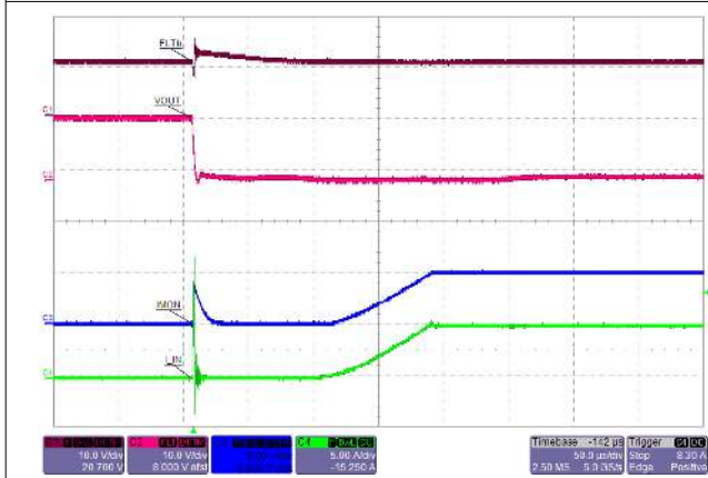
Figure 10-13. Hot Short: Fast Trip and Current Regulation
