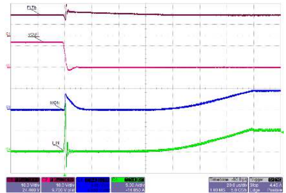
R_{(FLT)} = 100\text{ k}\Omega R_{(IMON)} = 16.9\text{ k}\Omega R_{(ILIM)} = 17.8\text{ k}\Omega Figure 7-40. Hot-Short: Fast Trip Response and Current Regulation
