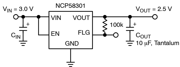
Figure 1. Fixed 2.5 Regulator with Error Flag
