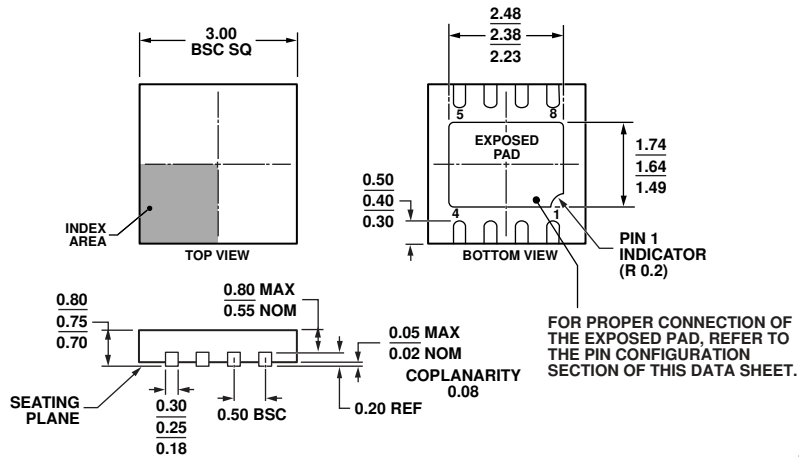
Figure 58. 8-Lead Lead Frame Chip Scale Package [LFCSWP] 3 mm x 3 mm Body, Very Very Thin, Dual Lead (CP-8-5)
