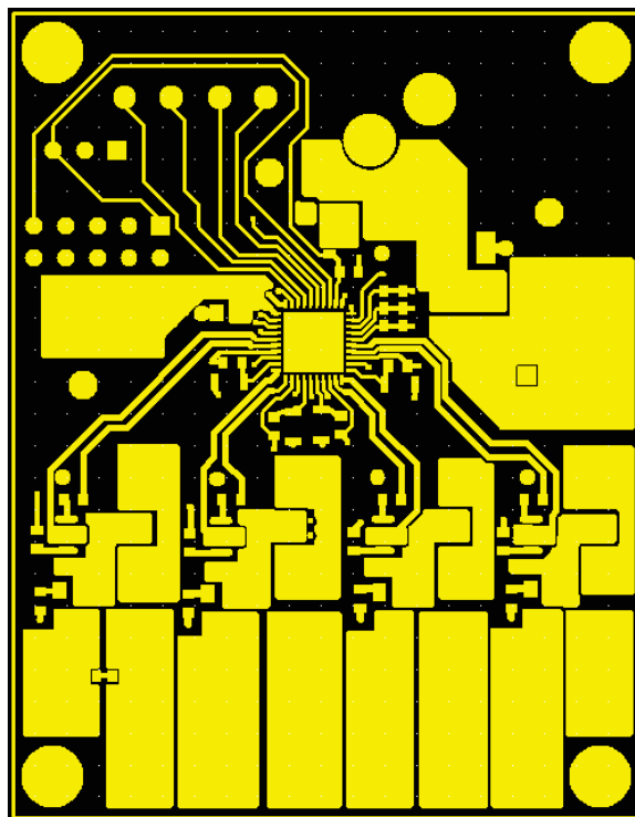
Figure 9: Bottom Layer
