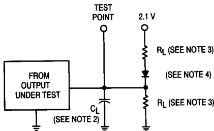
LOAD CIRCUIT FOR 3-STATE OUTPUT
