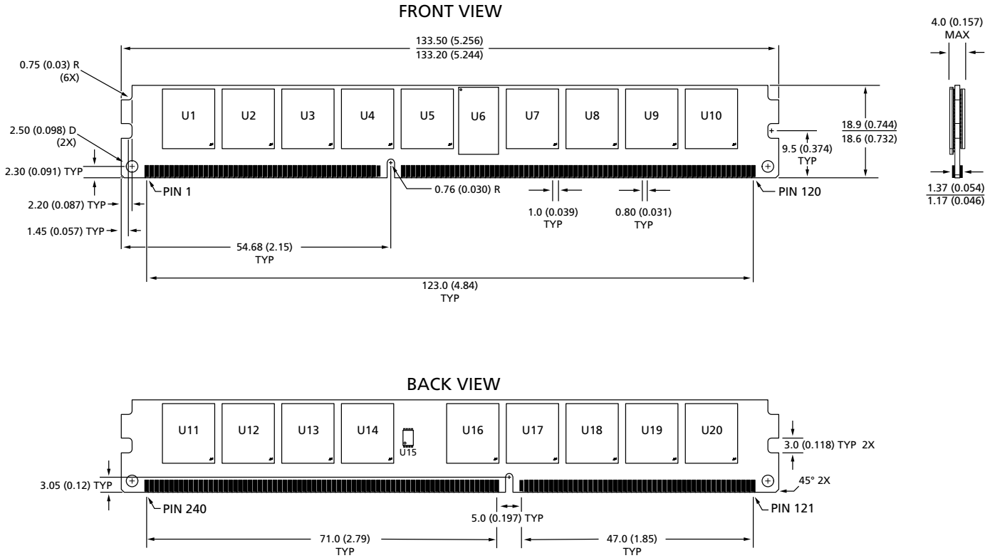
Figure 3: 240-Pin DDR3 RDIMM
