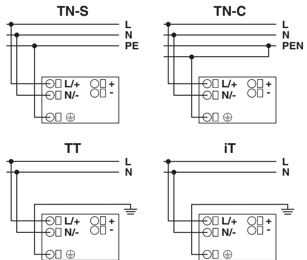
Figure 16 Network types
