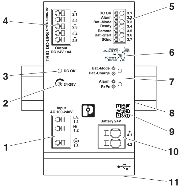
Figure 1 Function elements
