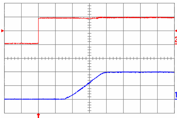
Fig. 1.0V.5: Turn-on transient for V_{out} = 1.0\text{ V} with the application of Enable signal at full rated load current (resistive) and 100\text{ }\mu\text{F} external capacitance at V_{in} = 5\text{ V} . Top trace: Enable signal (2 V/div.); Bottom trace: output voltage (500 mV/div.); Time scale: 2 ms/div.
