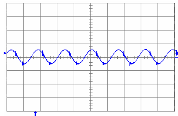
Fig. 1.0V.6: Output voltage ripple (20 mV/div.) at full rated load current into a resistive load with external capacitance 100\text{ }\mu\text{F} ceramic + 1\text{ }\mu\text{F} ceramic and V_{in} = 5\text{ V} for V_{out} = 1.0\text{ V} . Time scale: 2 \mu\text{s} /div.
