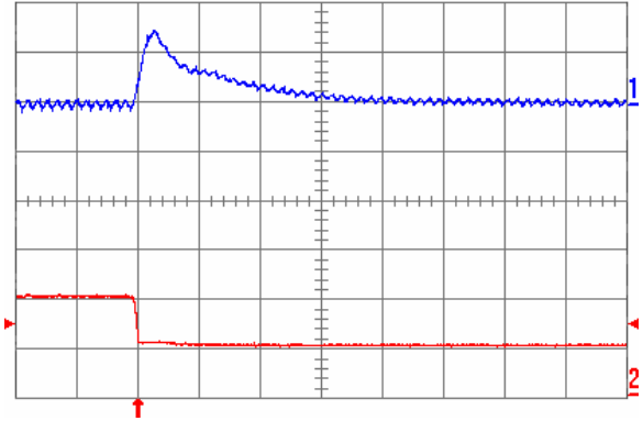
Fig. 1.0V.8: Output voltage response for V_{out} = 1.0\text{ V} to negative load current step change from 10 A to 5 A with slew rate of -5\text{ A}/\mu\text{s} at V_{in} = 5\text{ V} . Top trace: output voltage (100 mV/div.); Bottom trace: load current (5 A/div.). C_o = 100\text{ }\mu\text{F} ceramic + 1\text{ }\mu\text{F} ceramic. Time scale: 20\text{ }\mu\text{s}/\text{div} .
