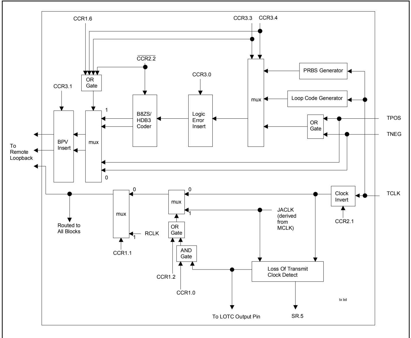
Figure 1-3. Transmit Logic
