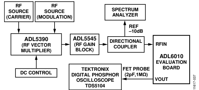
Figure 39. Hardware Configuration for Envelope Output Response Measurement
