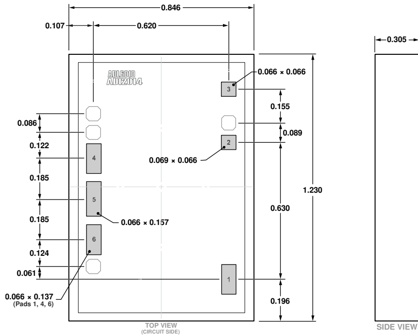
Figure 51. 6-Pad Bare Die [CHIP] (C-6-14) Dimensions shown in millimeters
