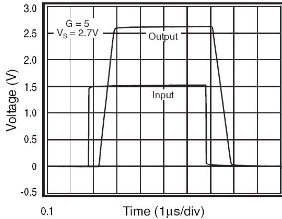
Figure 31. Overdrive Recovery
