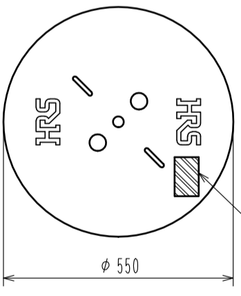
2 STYLE AND DIMENSION OF REEL
