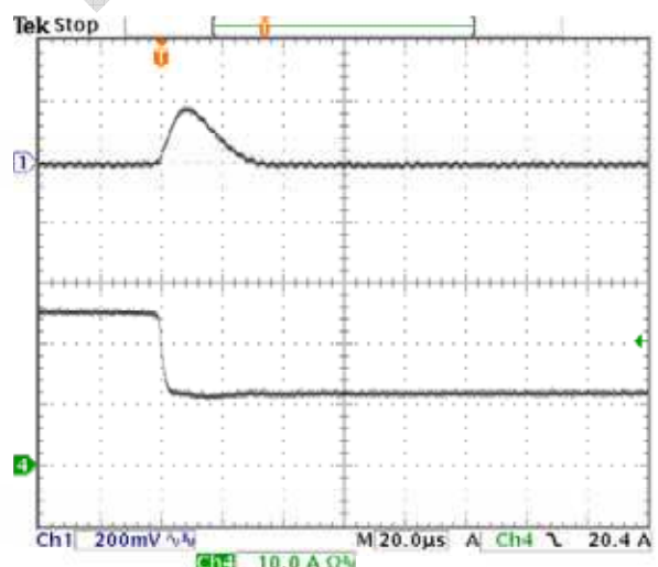
Fig-2.5V-7: Output voltage response for V_{out}=2.5V to positive load current step-change from 25A to 12.5A with slew rate of -5A/\mu s at V_{in}=12.0V . C_o=47\mu F \times 2 ceramic. Top trace: output voltage (200mV/div.) Bottom trace: load current (10A/div.) Time scale: 20μs/div.
