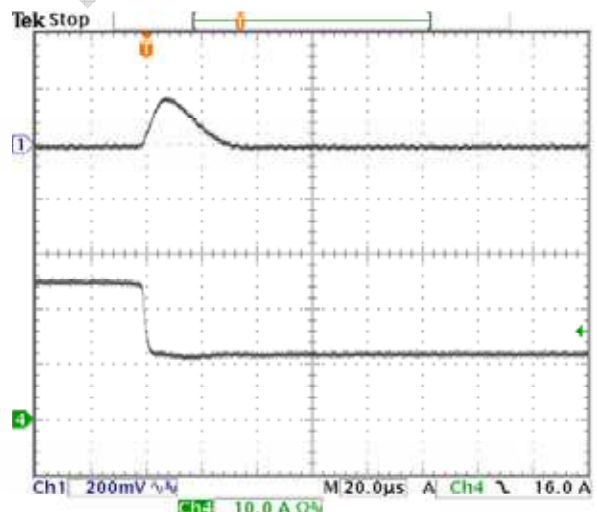
Fig-2.0V-7: Output voltage response for V_{out}=2.0V to positive load current step-change from 25A to 12.5A with slew rate of -5A/\mu s at V_{in}=12.0V . C_o=47\mu F \times 2 ceramic. Top trace: output voltage (200mV/div.) Bottom trace: load current (10A/div.) Time scale: 20μs/div.
