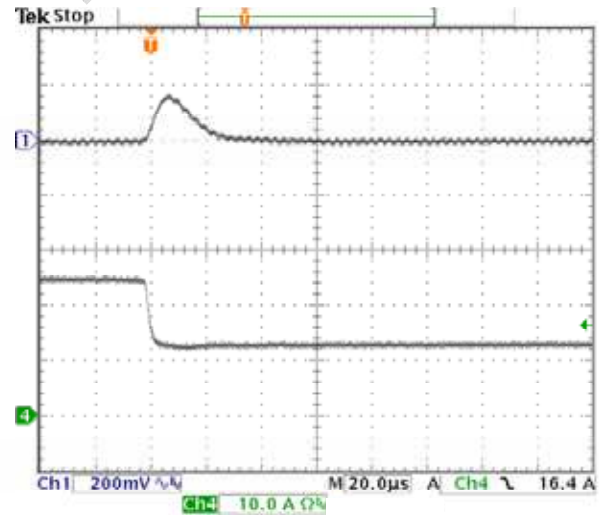
Fig-3.3V-7: Output voltage response for V_{out}=3.3V to positive load current step-change from 25A to 12.5A with slew rate of -5A/\mu s at V_{in}=12.0V . C_o=47\mu F \times 2 ceramic. Top trace: output voltage (200mV/div.) Bottom trace: load current (10A/div.) Time scale: 20µs/div.
