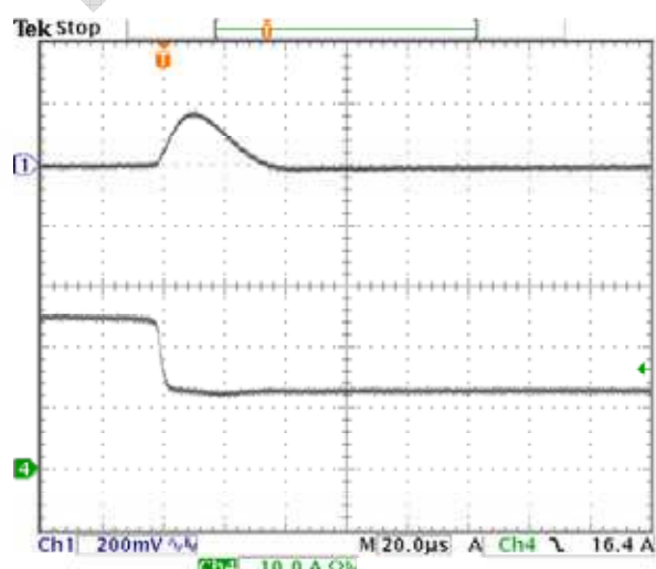
Fig-1.0V-7: Output voltage response for V_{out}=1.0V to positive load current step-change from 25A to 12.5A with slew rate of -5A/\mu s at V_{in}=12.0V . C_o=47\mu F \times 2 ceramic. Top trace: output voltage (200mV/div.) Bottom trace: load current (10A/div.) Time scale: 20μs/div.
