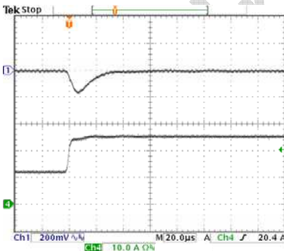
Fig-2.5V-6: Output voltage response for V_{out}=2.5V to positive load current step-change from 12.5A to 25A with slew rate of 5A/\mu s at V_{in}=12.0V . C_o=47\mu F \times 2 ceramic. Top trace: output voltage (200mV/div.) Bottom trace: load current (10A/div.) Time scale: 20μs/div.
