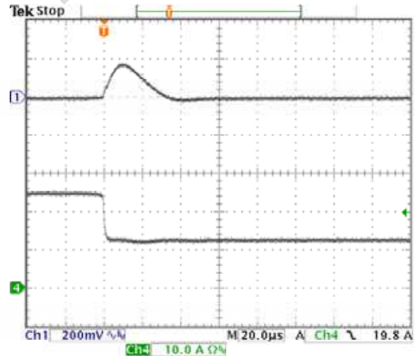
Fig-1.2V-7: Output voltage response for V_{out}=1.2V to positive load current step-change from 25A to 12.5A with slew rate of -5A/\mu s at V_{in}=12.0V . C_o=47\mu F \times 2 ceramic. Top trace: output voltage (200mV/div.) Bottom trace: load current (10A/div.) Time scale: 20μs/div.
