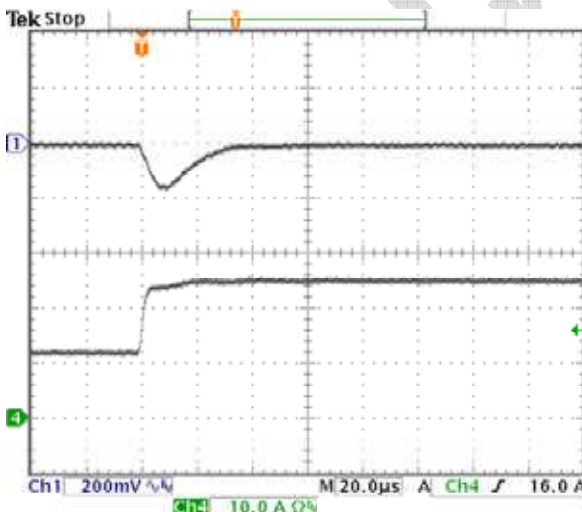
Fig-2.0V-6: Output voltage response for V_{out}=2.0V to positive load current step-change from 12.5A to 25A with slew rate of 5A/\mu s at V_{in}=12.0V . C_o=47\mu F \times 2 ceramic. Top trace: output voltage (200mV/div.) Bottom trace: load current (10A/div.) Time scale: 20μs/div.
