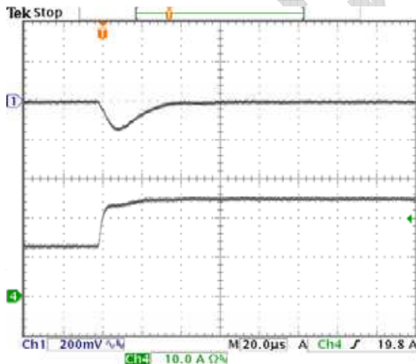
Fig-1.2V-6: Output voltage response for V_{out}=1.2V to positive load current step-change from 12.5A to 25A with slew rate of 5A/\mu s at V_{in}=12.0V . C_o=47\mu F \times 2 ceramic. Top trace: output voltage (200mV/div.) Bottom trace: load current (10A/div.) Time scale: 20μs/div.
