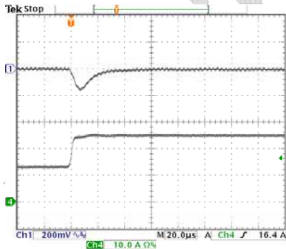
Fig-3.3V-6: Output voltage response for V_{out}=3.3V to positive load current step-change from 12.5A to 25A with slew rate of 5A/\mu s at V_{in}=12.0V . C_o=47\mu F \times 2 ceramic. Top trace: output voltage (200mV/div.) Bottom trace: load current (10A/div.) Time scale: 20µs/div.
