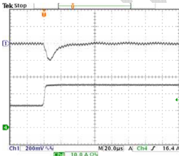
Fig-5.0V-6: Output voltage response for V_{out}=5.0V to positive load current step-change from 12.5A to 25A with slew rate of 5A/\mu s at V_{in}=12.0V . C_o=47\mu F \times 2 ceramic. Top trace: output voltage (200mV/div.) Bottom trace: load current (10A/div.) Time scale: 20µs/div.
