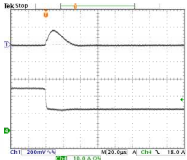
Fig-1.5V-7: Output voltage response for V_{out}=1.5V to positive load current step-change from 25A to 12.5A with slew rate of -5A/\mu s at V_{in}=12.0V . C_o=47\mu F \times 2 ceramic. Top trace: output voltage (200mV/div.) Bottom trace: load current (10A/div.) Time scale: 20μs/div.
