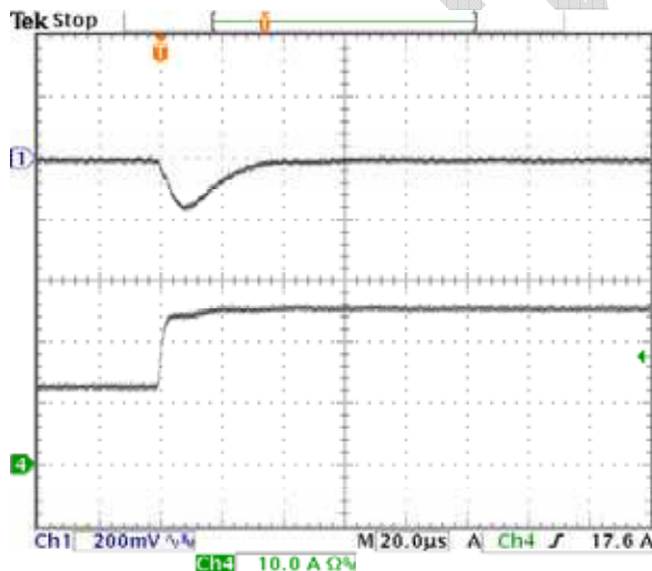
Fig-1.8V-6: Output voltage response for V_{out}=1.8V to positive load current step-change from 12.5A to 25A with slew rate of 5A/\mu s at V_{in}=12.0V . C_o=47\mu F \times 2 ceramic. Top trace: output voltage (200mV/div.) Bottom trace: load current (10A/div.) Time scale: 20μs/div.
