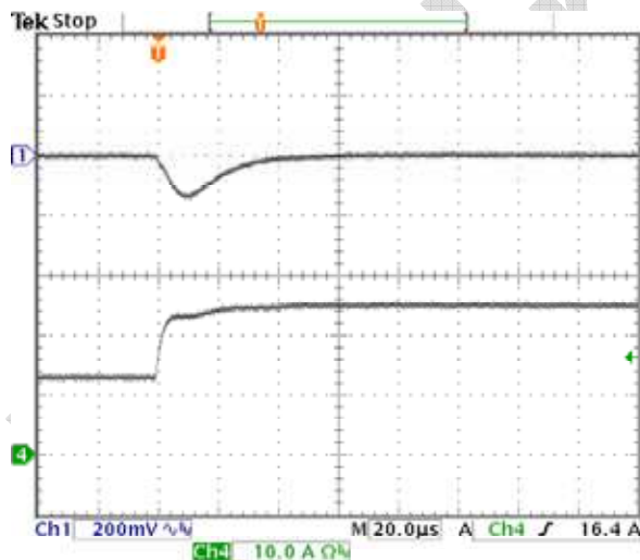
Fig-1.0V-6: Output voltage response for V_{out}=1.0V to positive load current step-change from 12.5A to 25A with slew rate of 5A/\mu s at V_{in}=12.0V . C_o=47\mu F \times 2 ceramic. Top trace: output voltage (200mV/div.) Bottom trace: load current (10A/div.) Time scale: 20μs/div.
