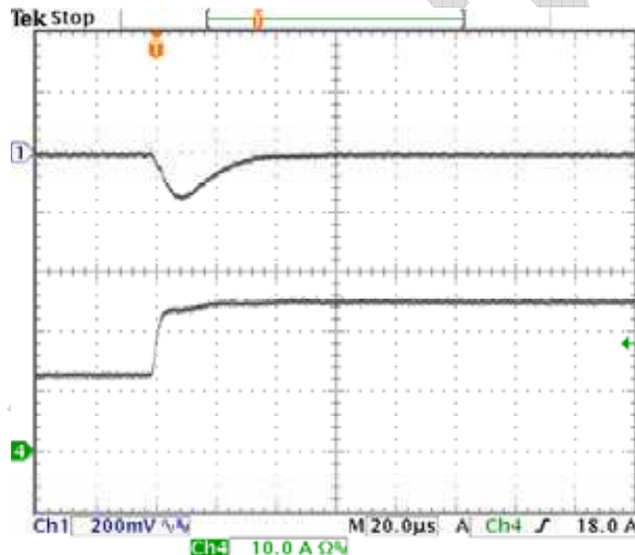
Fig-1.5V-6: Output voltage response for V_{out}=1.5V to positive load current step-change from 12.5A to 25A with slew rate of 5A/\mu s at V_{in}=12.0V . C_o=47\mu F \times 2 ceramic. Top trace: output voltage (200mV/div.) Bottom trace: load current (10A/div.) Time scale: 20μs/div.
