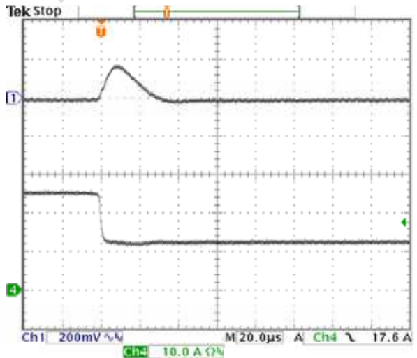
Fig-1.8V-7: Output voltage response for V_{out}=1.8V to positive load current step-change from 25A to 12.5A with slew rate of -5A/\mu s at V_{in}=12.0V . C_o=47\mu F \times 2 ceramic. Top trace: output voltage (200mV/div.) Bottom trace: load current (10A/div.) Time scale: 20μs/div.
