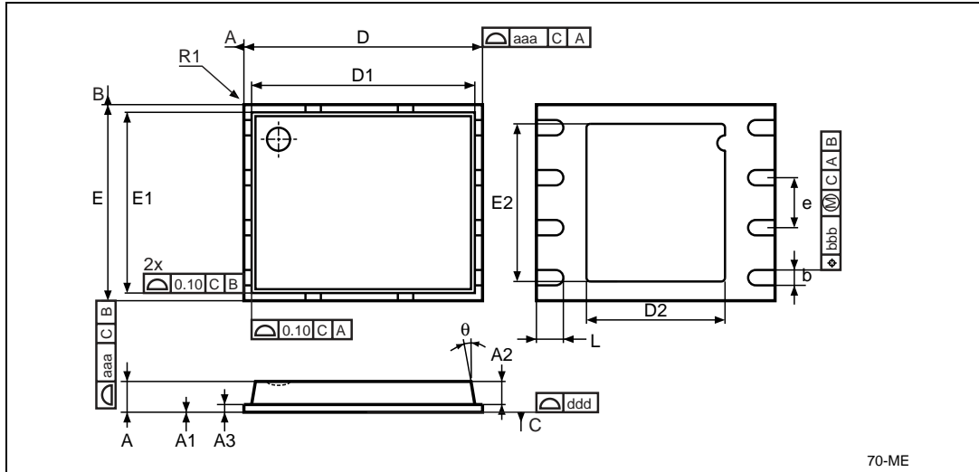
Figure 29. VFDFPN8 (MLP8) 8-lead Very thin Fine pitch Quad Flat Package No lead, 6 x 5 mm, package outline
