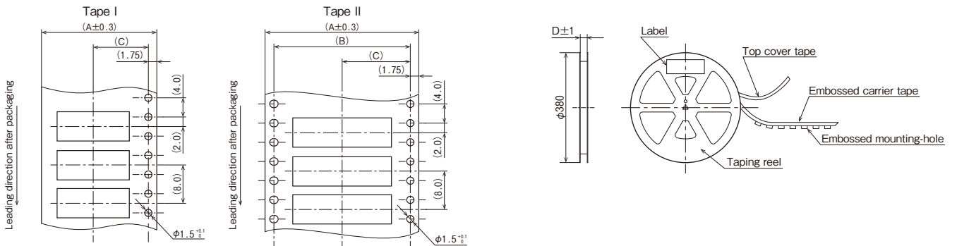
Dimension table
