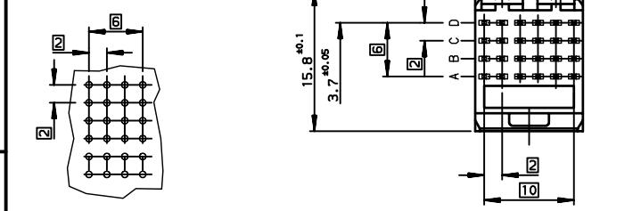
LAYOUT FOR P.C.B (PER 12mm LENGTH)
