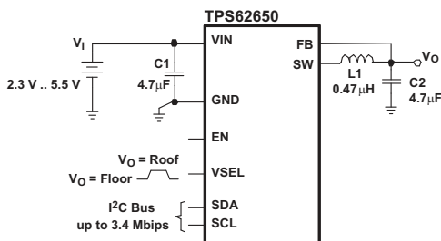
Figure 1. Typical Application
