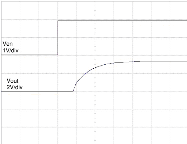
Time (20us/div)
