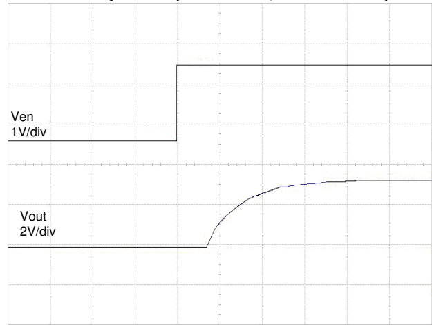
Time (20us/div)
