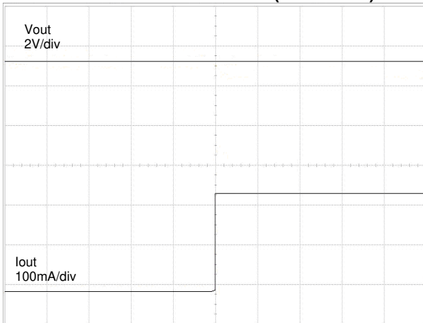
Time (50us/div)
