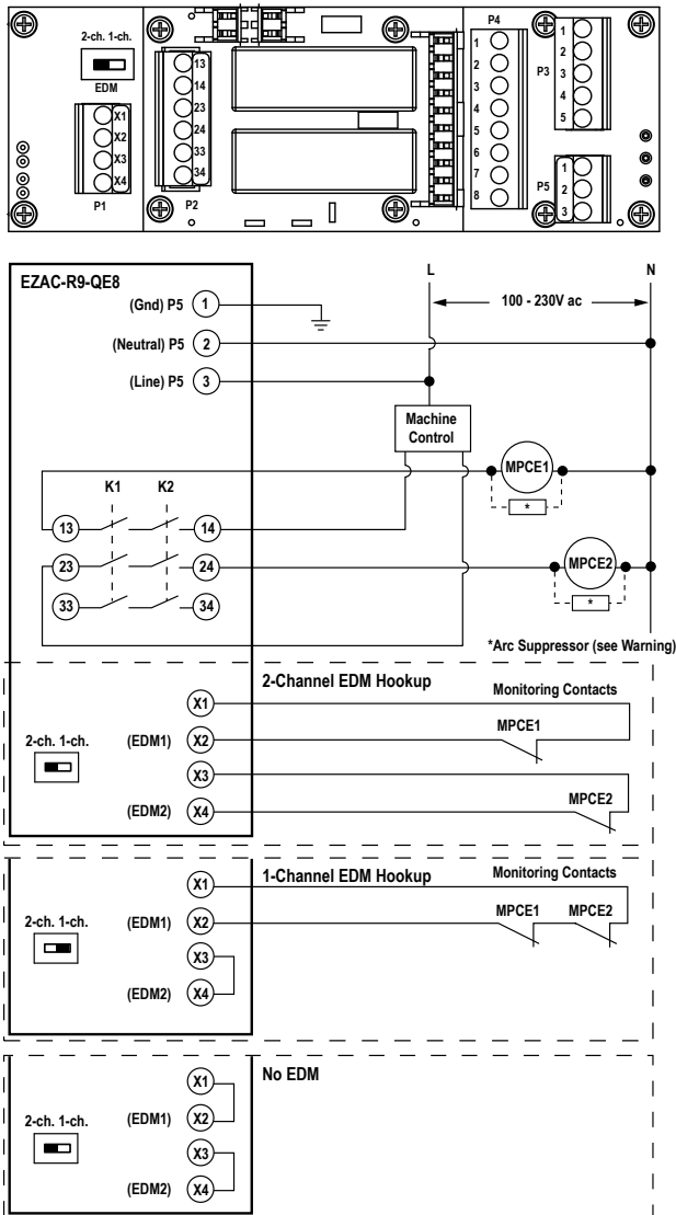
Figure 7. Wiring—model EZAC-R9-QE8
