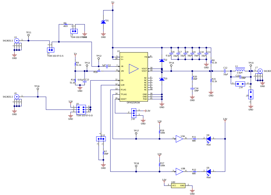
Figure 2. OPA521EVM Partial Schematic
