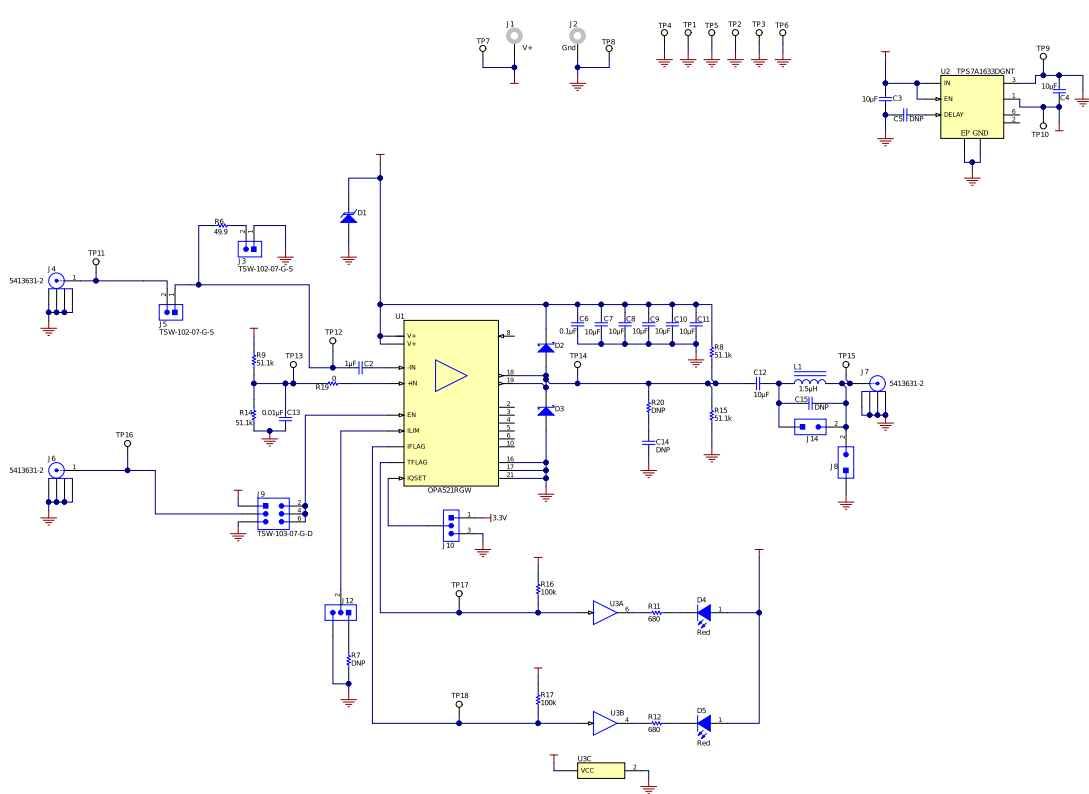
Figure 3. OPA521EVM Schematic
