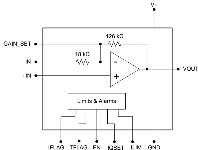
Figure 1. OPA521 Device Functional Block Diagram
