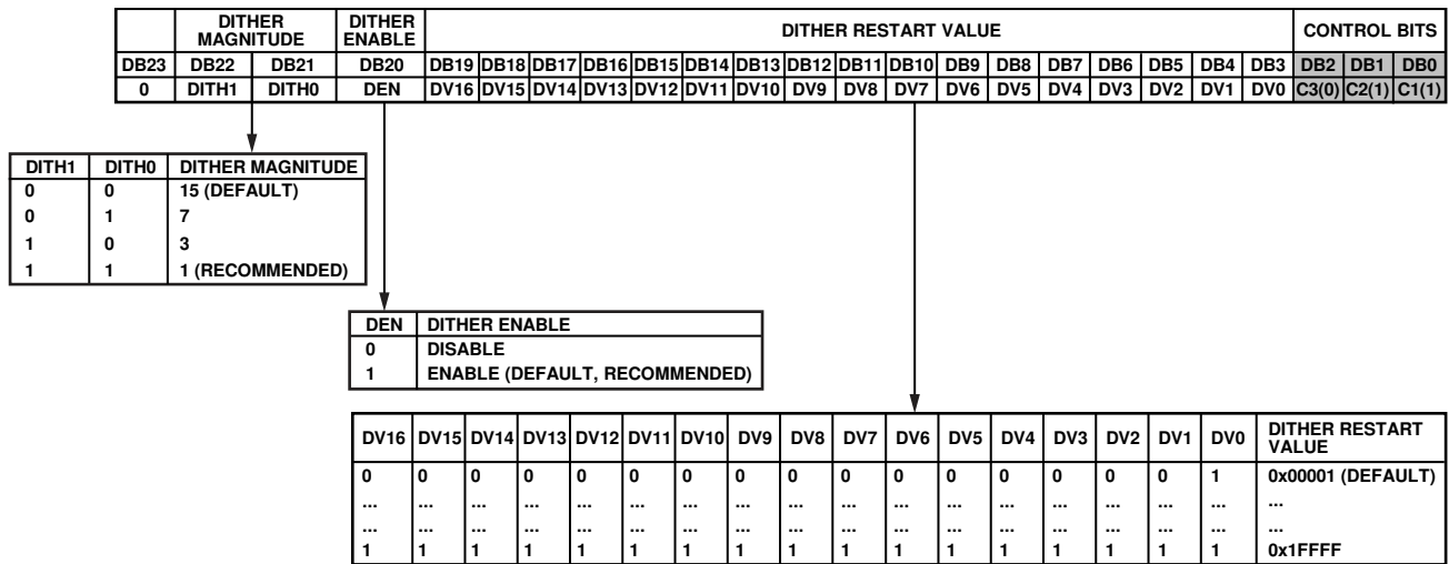
Figure 41. Register 3— \Sigma - \Delta Modulator Dither Control Register Map
